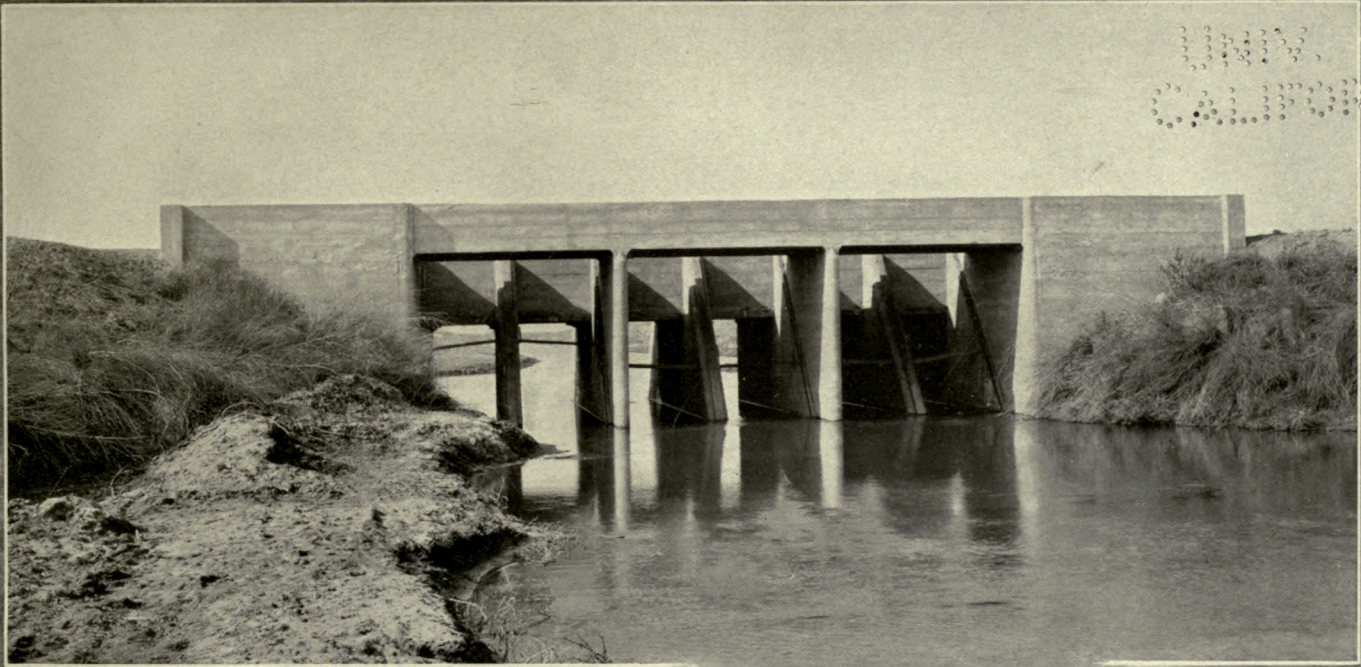
Another view of the Temple Slough weir. The roadway performs the double function of serving traffic and, through its weight, adding to the stability of the weir
