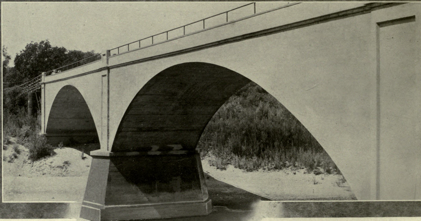
This substantial highway bridge spans the Stanislaus River near Modesto, connecting San Joaquin and Stanislaus Counties
