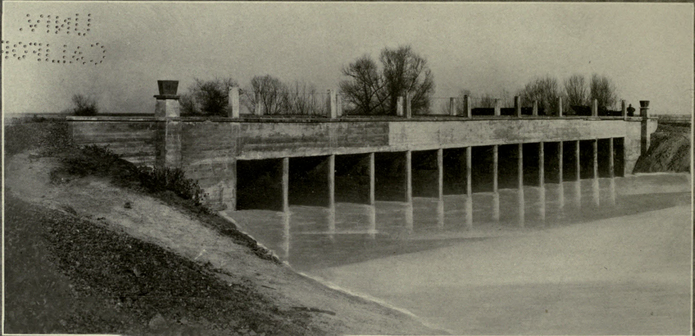
This combination bridge and weir crosses the slough which controls the water from Buena Vista Lake
