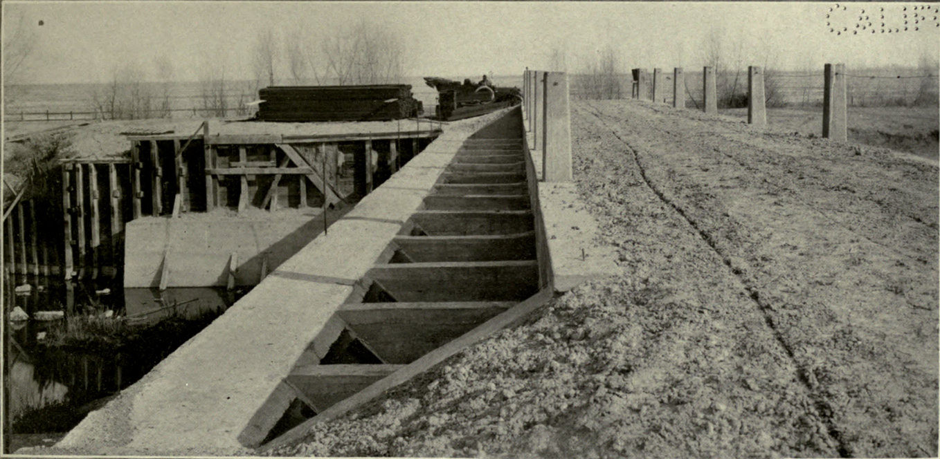
Another view of the Old Headquarters Weir, showing the roadway and at the left a concrete slab that can be used for a footwalk
