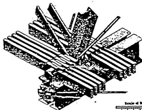
Connections of Lower Chord at A.
