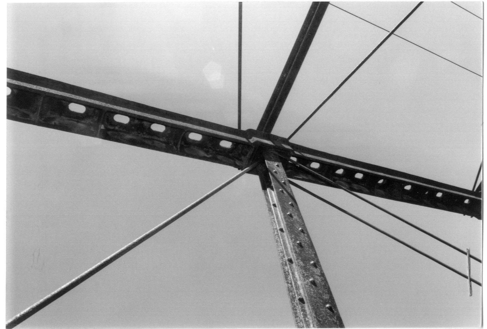
NW TRUSS, INTERMEDIATE UPPER PANEL POINT (7-24-85)
