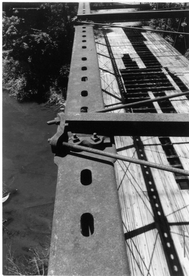
(SAME) FROM NE (7-24-85)
