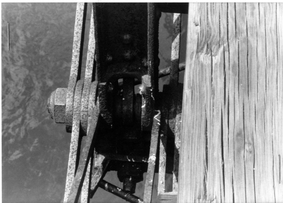
SE TRUSS LOWER CHORD PANEL POINT FROM ABOVE (8-14-86)
