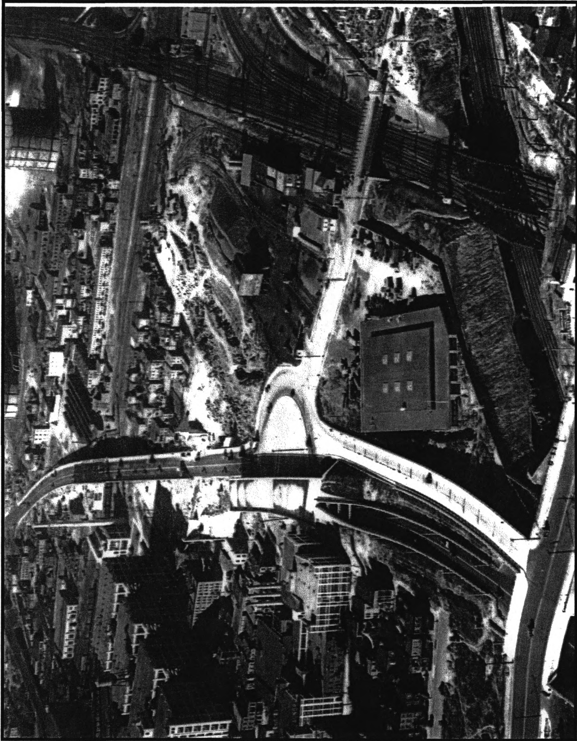
Figure 4. Ca. 1930 aerial view looking west at Tonnele Circle, west end of east section 2 of Route 1 Extension, and US Route 1. Overpass in foreground in JFK Boulevard. Courtesy of NJ Dept. of State: State Archives NJDOT Department of Transportation ca. 1920-1979 photographs filed by subject, Box 9, Jersey City Aerial Views folder.
