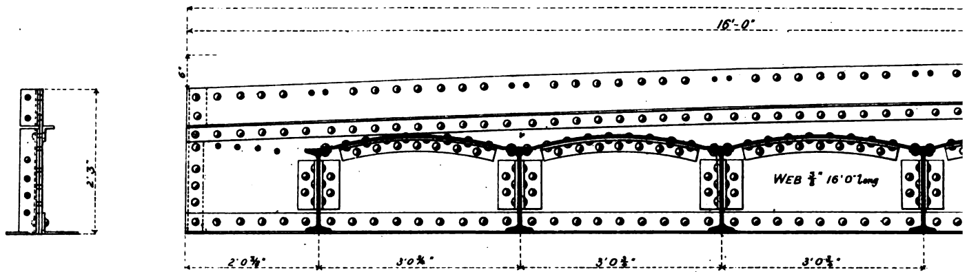
ELEVATION of SLIDING BEAM. END of IRON FLOORING.
