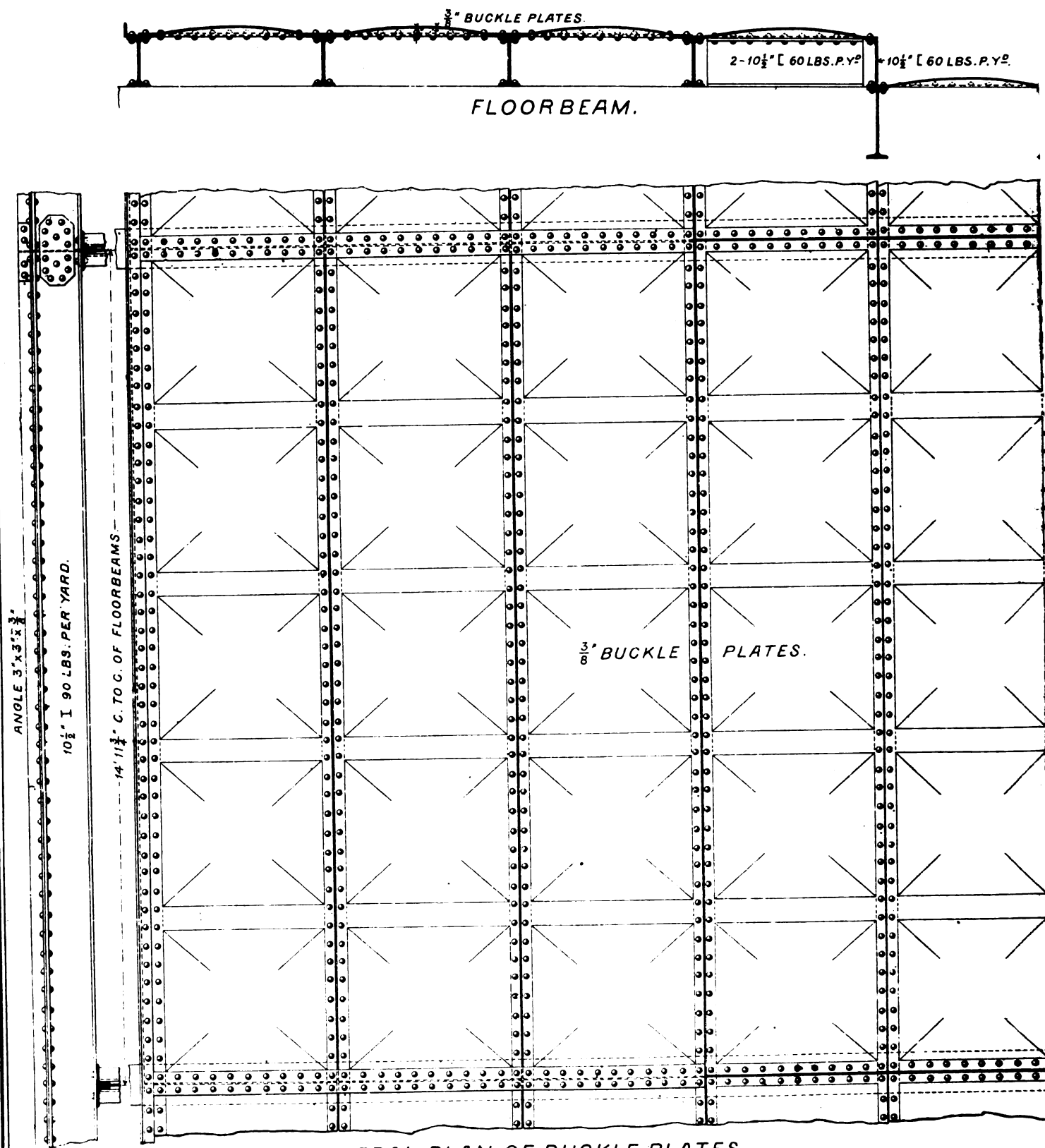
GENERAL PLAN OF BUCKLE PLATES.
