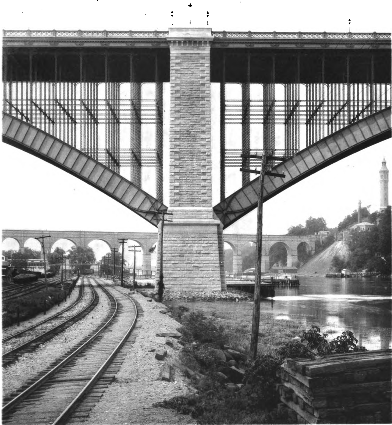
CENTRAL PIER, WASHINGTON BRIDGE.
