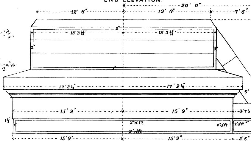
END ELEVATION.
