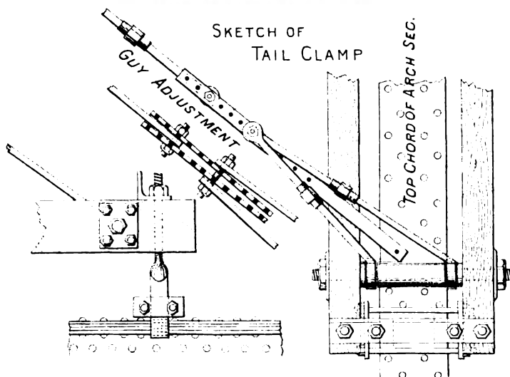
TRAVELING DERRICK AND DETAILS OF CLAMPS.
