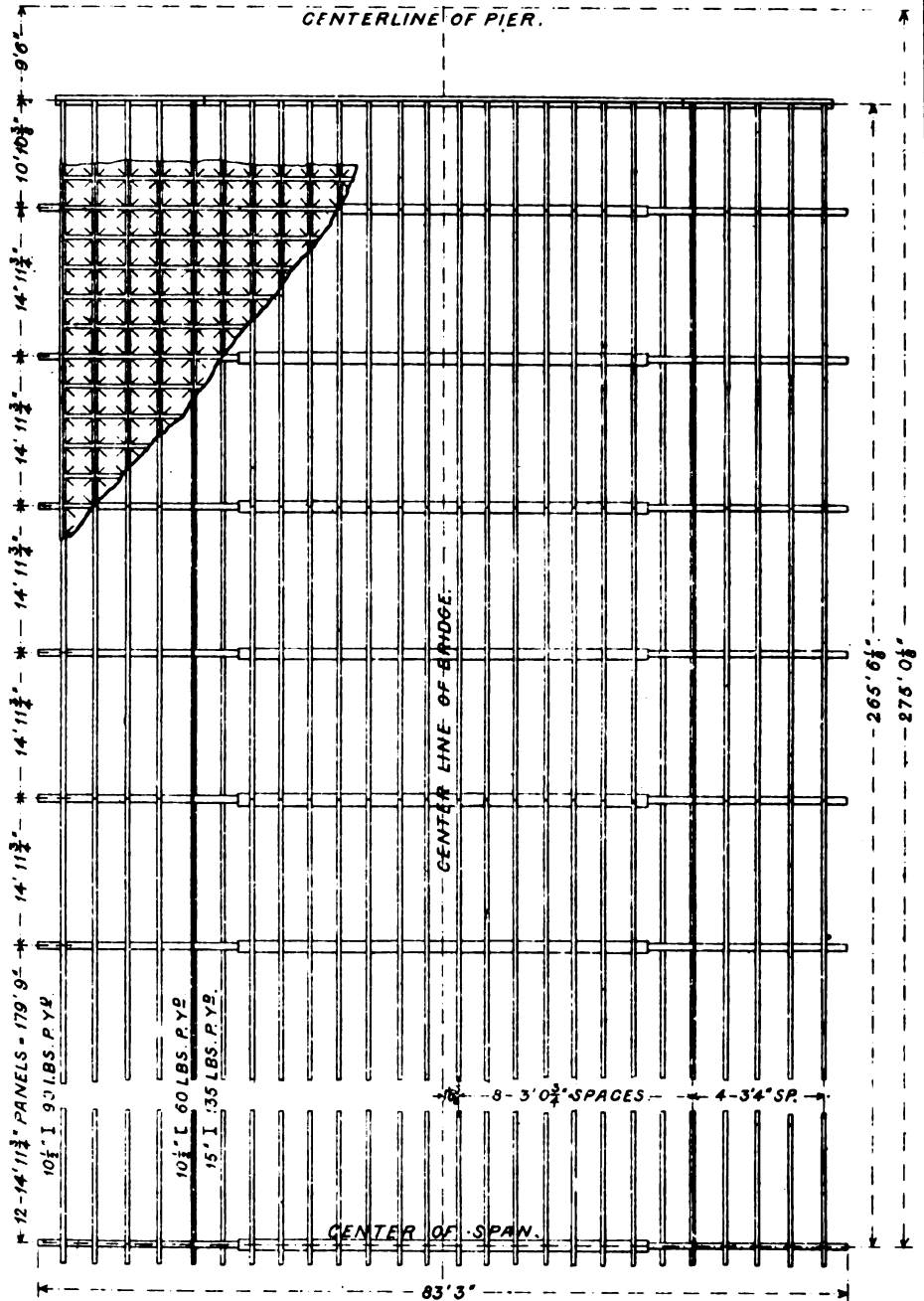
PLAN OF FLOORING.
