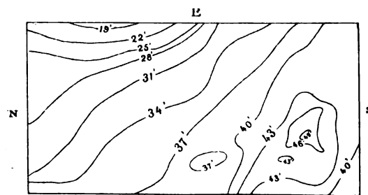
CONTOURS OF ROCK SURFACE UNDER CAISSON ELEVATIONS BELOW DATUM.
