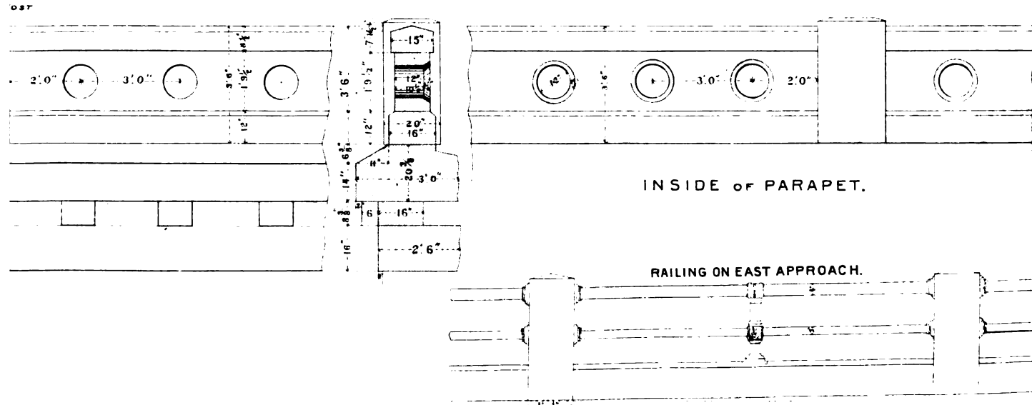
PARAPET OVER APPROACH.
