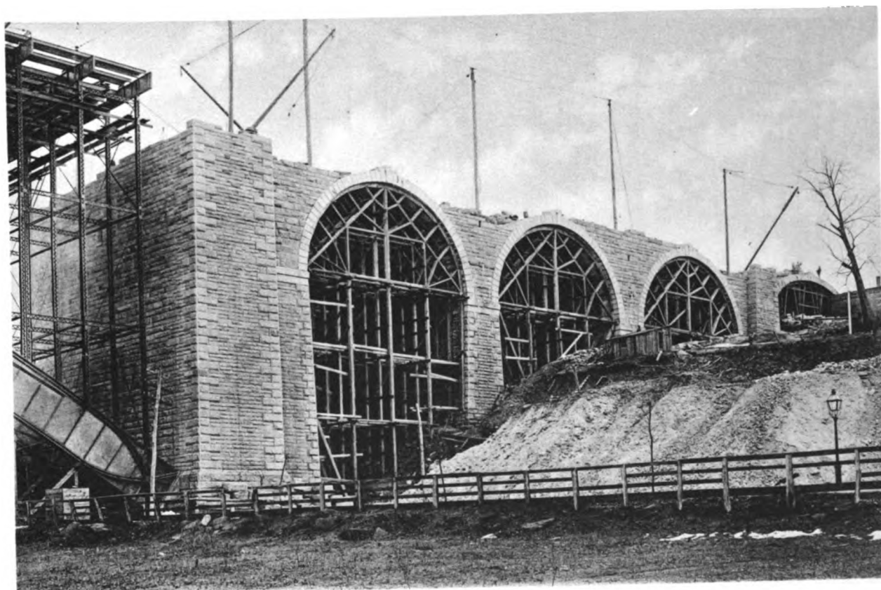
RIVER AND LAND SPANS, MARCH 23, 1888.
