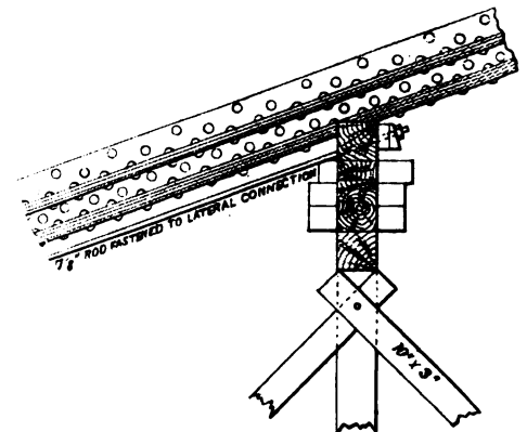
ARRANGMENT OF MOVABLE BLOCKS SUPPORTING ARCH SEGMENTS ON FALSE W
