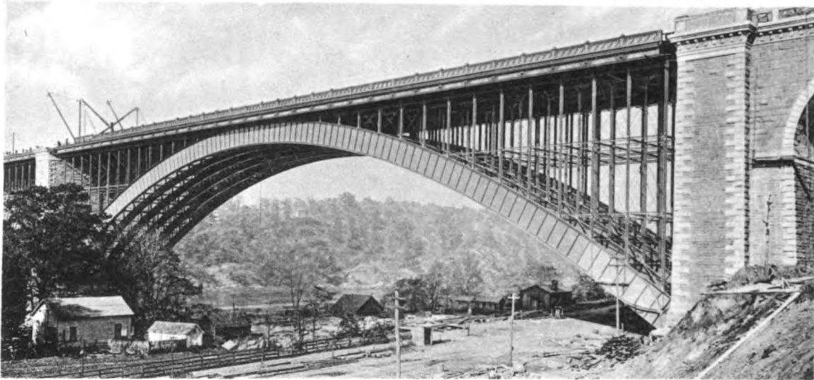
LANDSPAN, NOVEMBER 1, 1888.
