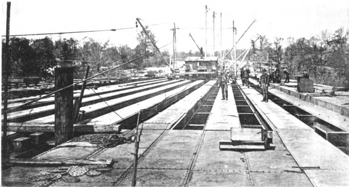
RIVER SPAN, MAY 18, 1888. SHOWING BUCKLE PLATES.
