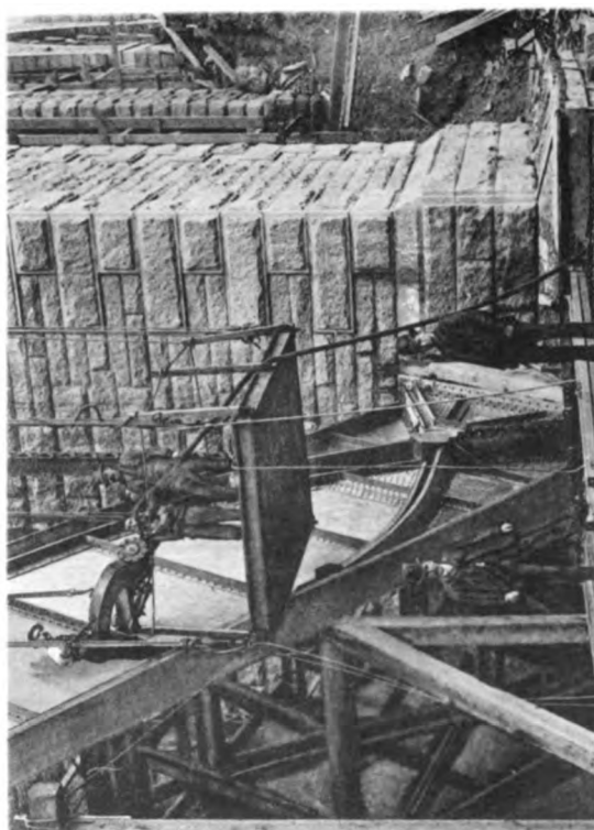
RIVETING MACHINE AT WORK.
