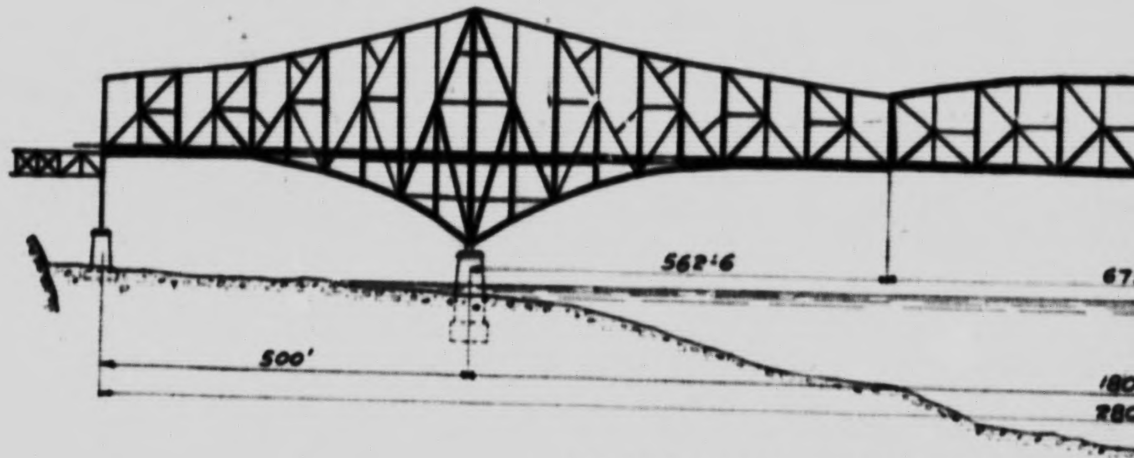
PHOENIX BRIDGE DESIGN
