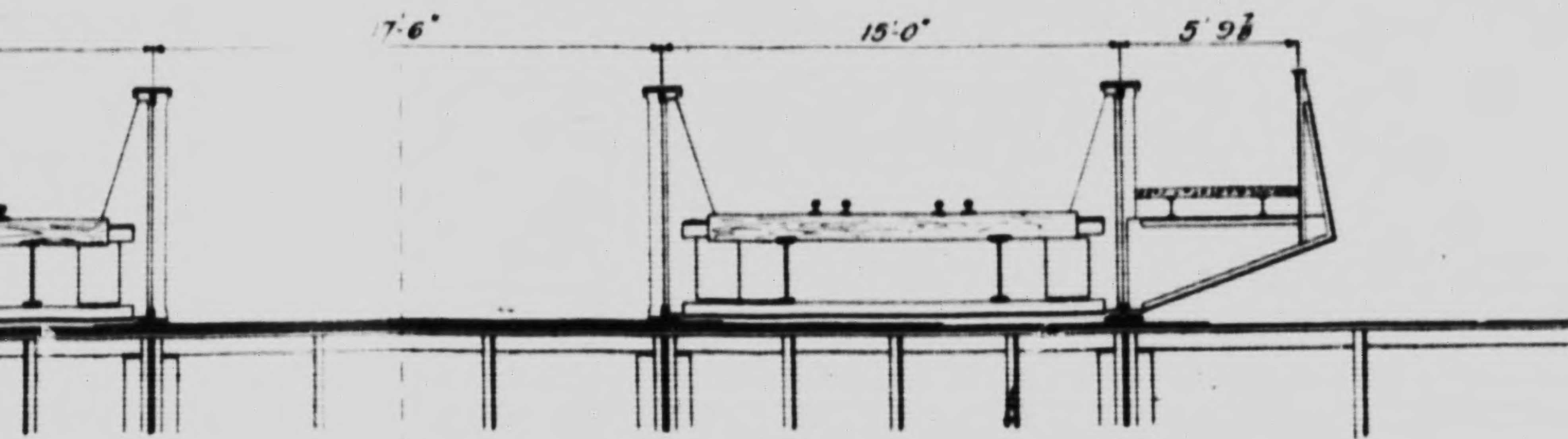
FLOOR AS BUILT
