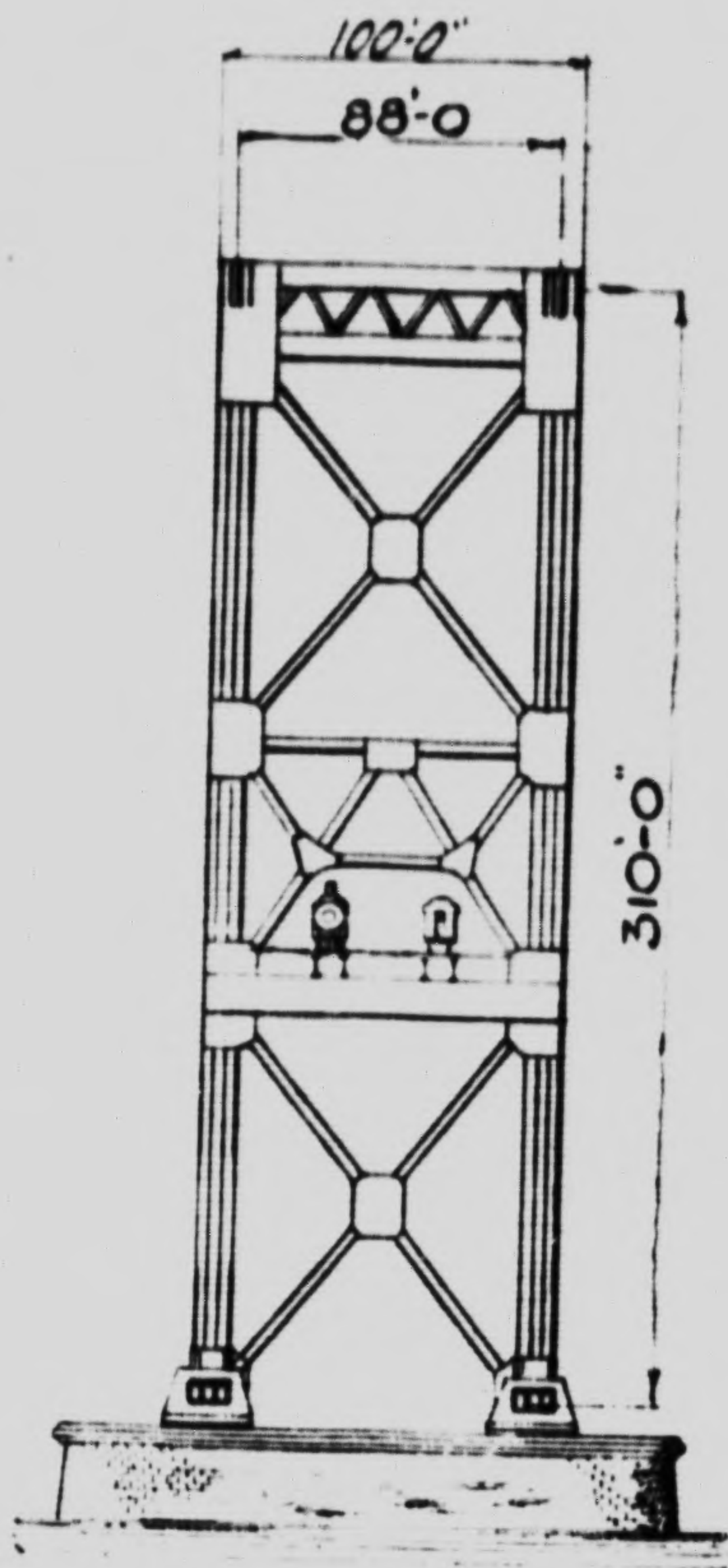
CROSS SECTION at MAIN PIERS
