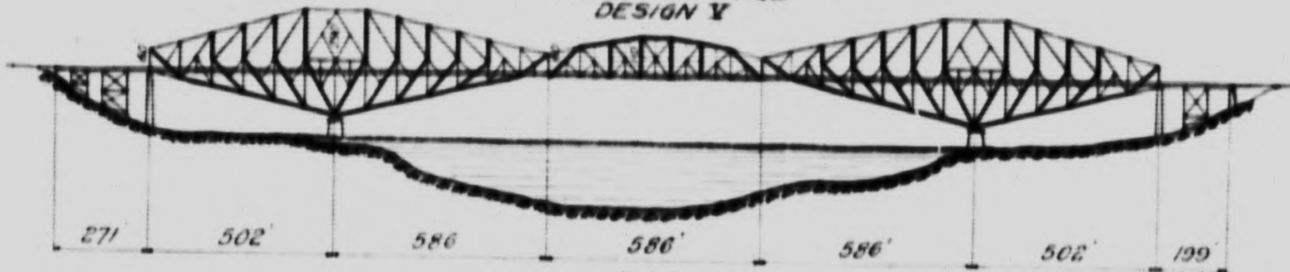
FIG 3 ST. LAWRENCE BRIDGE CO. LTD. QUEBEC BRIDGE DESIGN A-B-X
