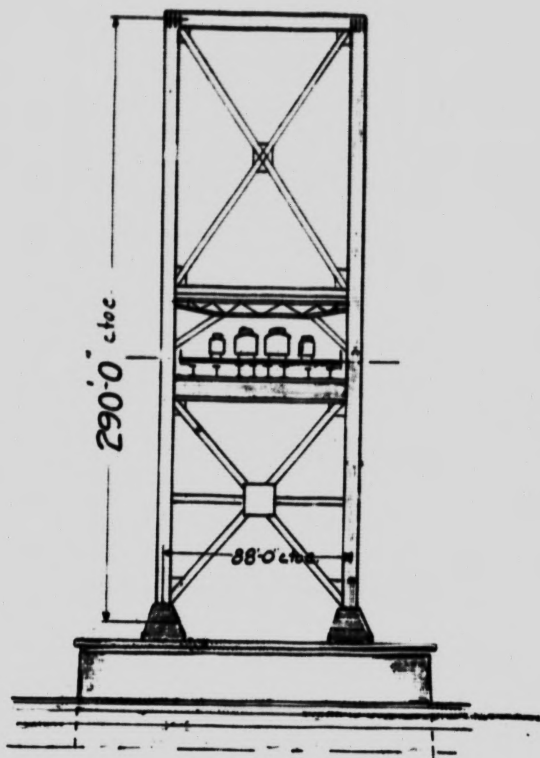
- DESIGN B - - Cross Section at Main Pier. -
