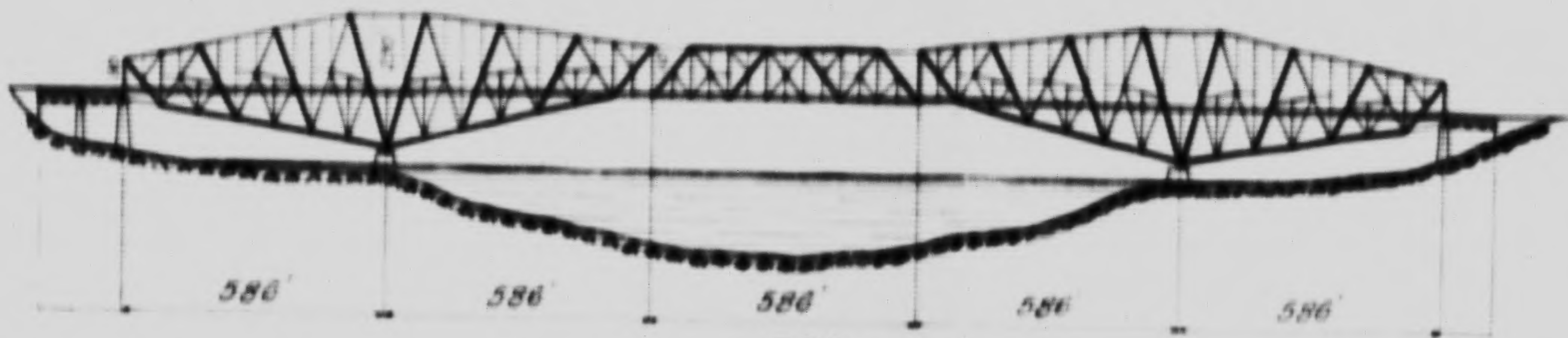
FIG 1 BOARD OF ENGINEERS QUEBEC BRIDGE DESIGN I
