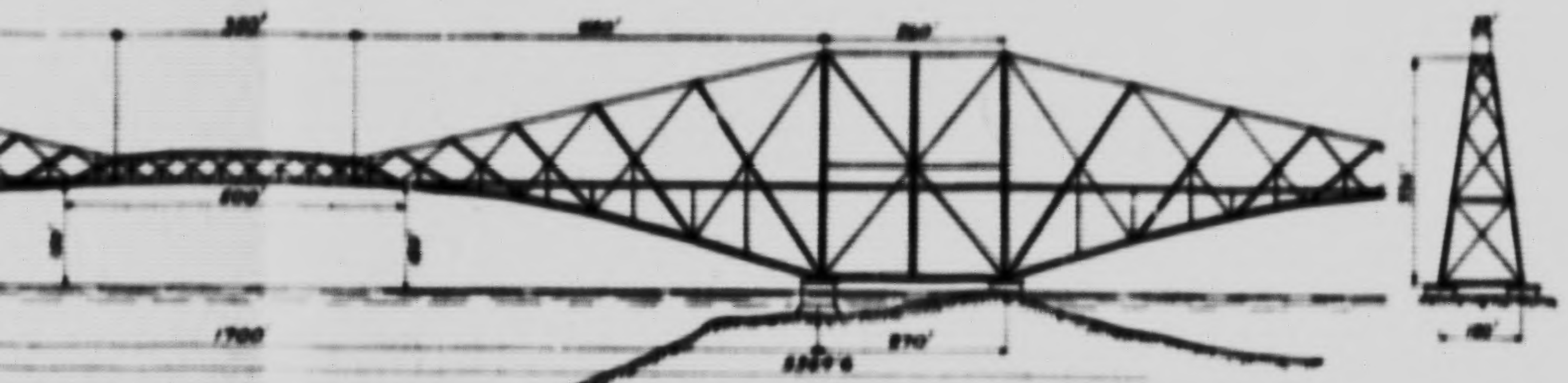
THE FORTH BRIDGE (NR. EDINBURGH SCOTLAND)
