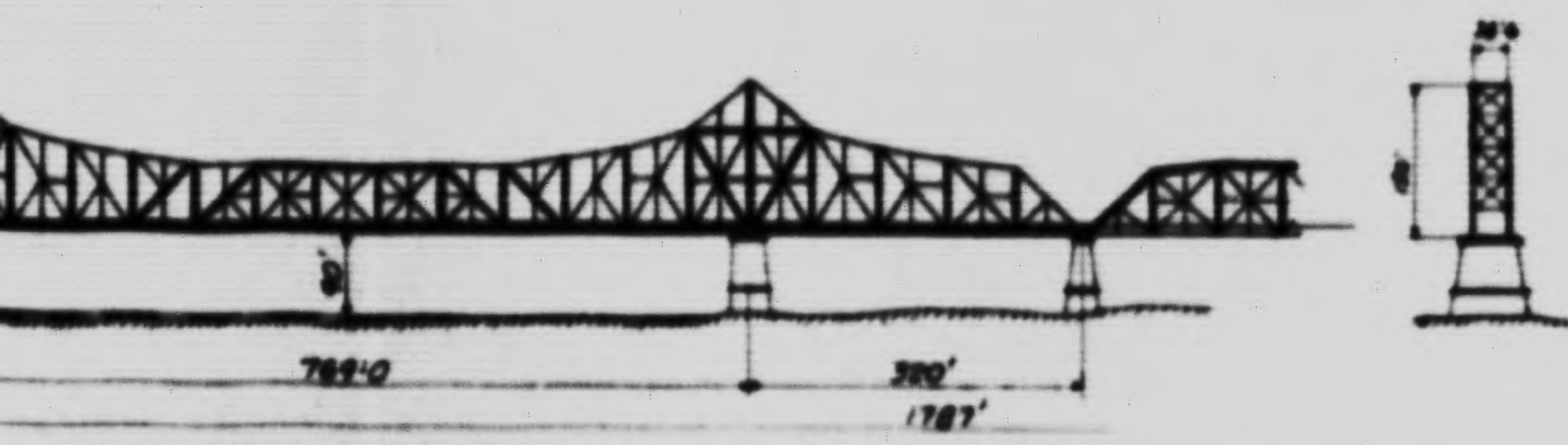
THE BEAVER BRIDGE (BEAVER PA)
