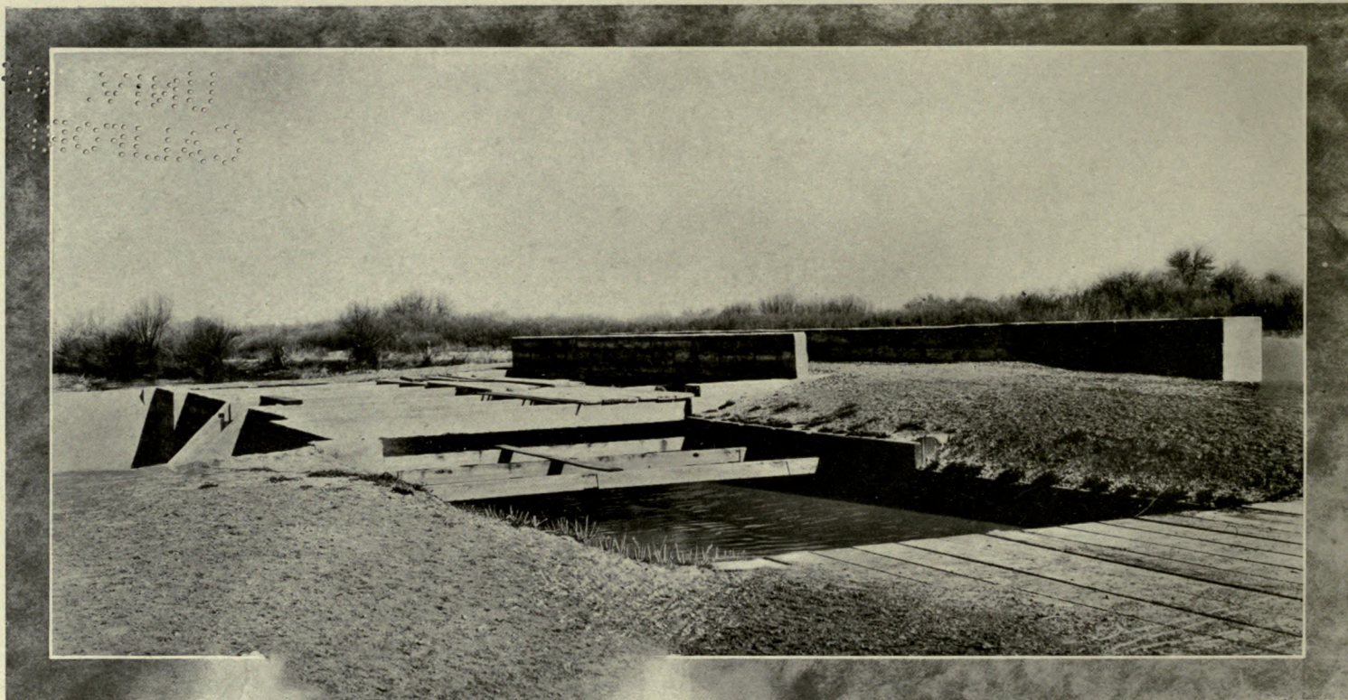
A combination weir, flume and bridge, showing the roadway and flume. Note volume of water in the flume
