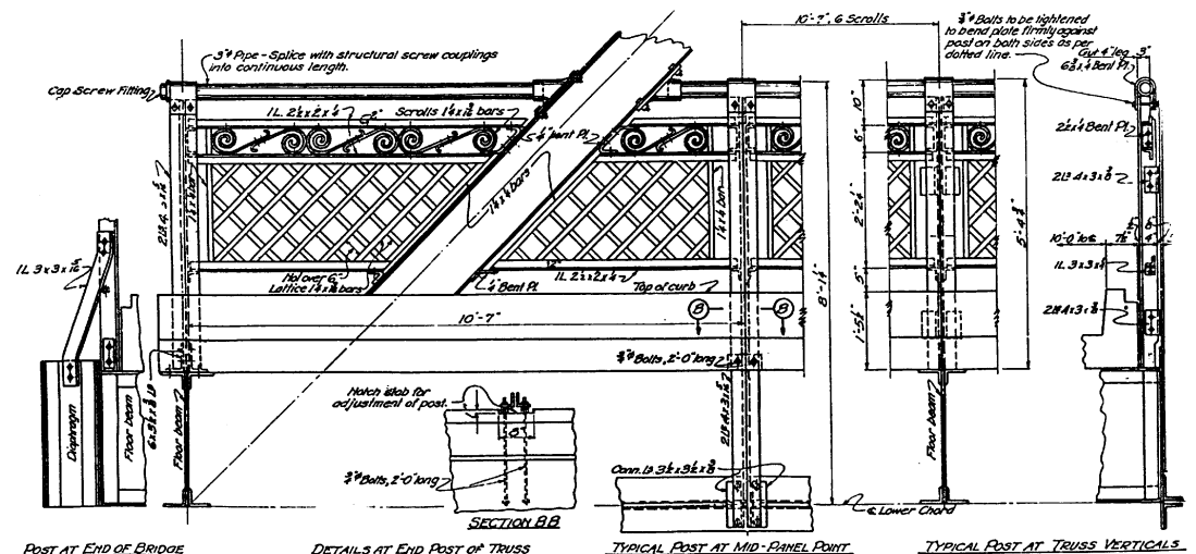
TYPICAL DETAILS OF HANDRAIL FOR WEST SIDE OF BRIDGE
