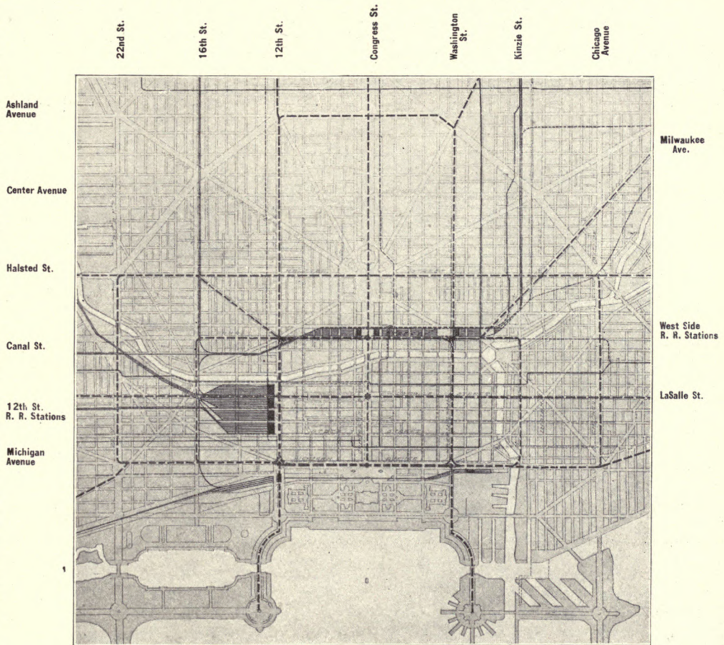
CHICAGO. Diagram of city center, showing the proposed arrangement of railroad passenger stations, the complete traction system, including rapid transit, subway and elevated roads, and the circuit subway line.
