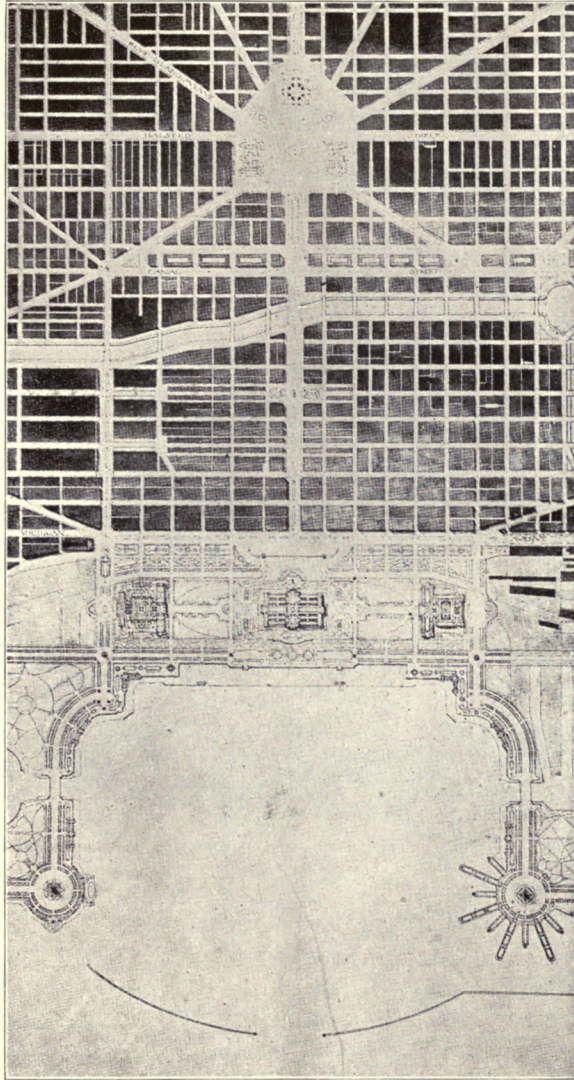
CHICAGO. The business center of the city within the first circuit boulevard, showing the proposed grand east-and-west axis and its relation to Grant Park and the yacht harbor; the railway terminals schemes on the south and west sides, and the Civic Center.
