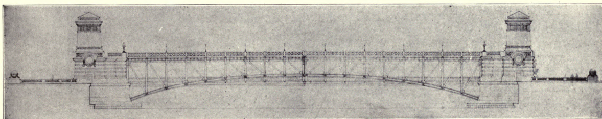
Proposed double deck bridge for north and south boulevard connection Michigan Avenue and Michigan Avenue projected.
