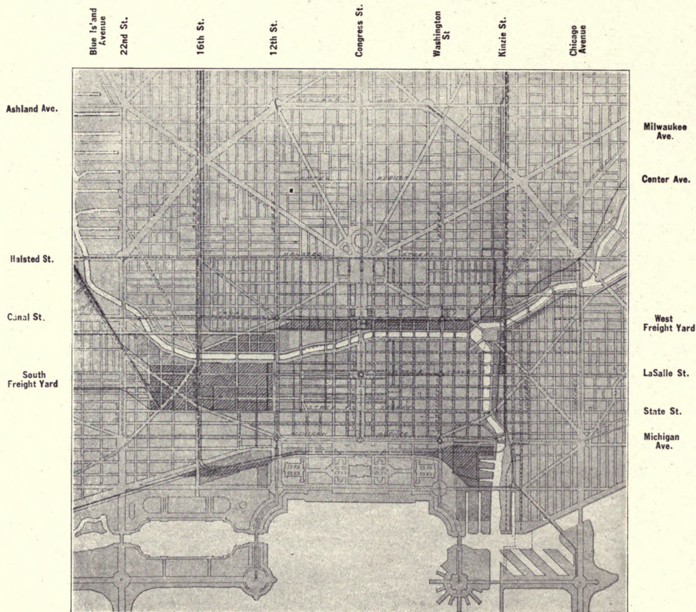
CHICAGO. Diagram of the city center, showing the general location of existing freight yards and railroad lines, the present tunnel system and proposed circuit, and connections for all these services, running to the central clearing yards.
