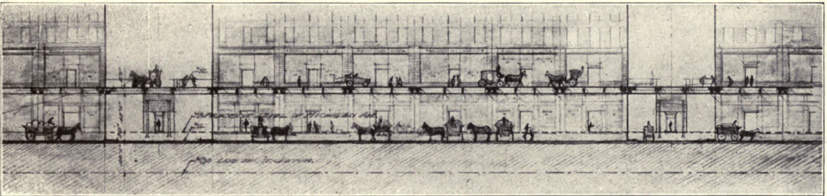
Section through Michigan Avenue between Lake Street and South Water Street looking West, showing raised street with upper and lower levels, with crossings at Lake and South Water Streets. This illustration shows store entrances on upper level directly off the sidewalk, also showing basement entrances on lower or grade level where shipping and heavy teaming will be done. In contemplating this drawing it must be remembered buildings have been effaced on the East side, the purpose being merely to show to the mind's eye the two levels in operation. [Note: Since this drawing was made, it has been decided to have the structural elevation commence at Lake Street instead of at Randolph Street.]
