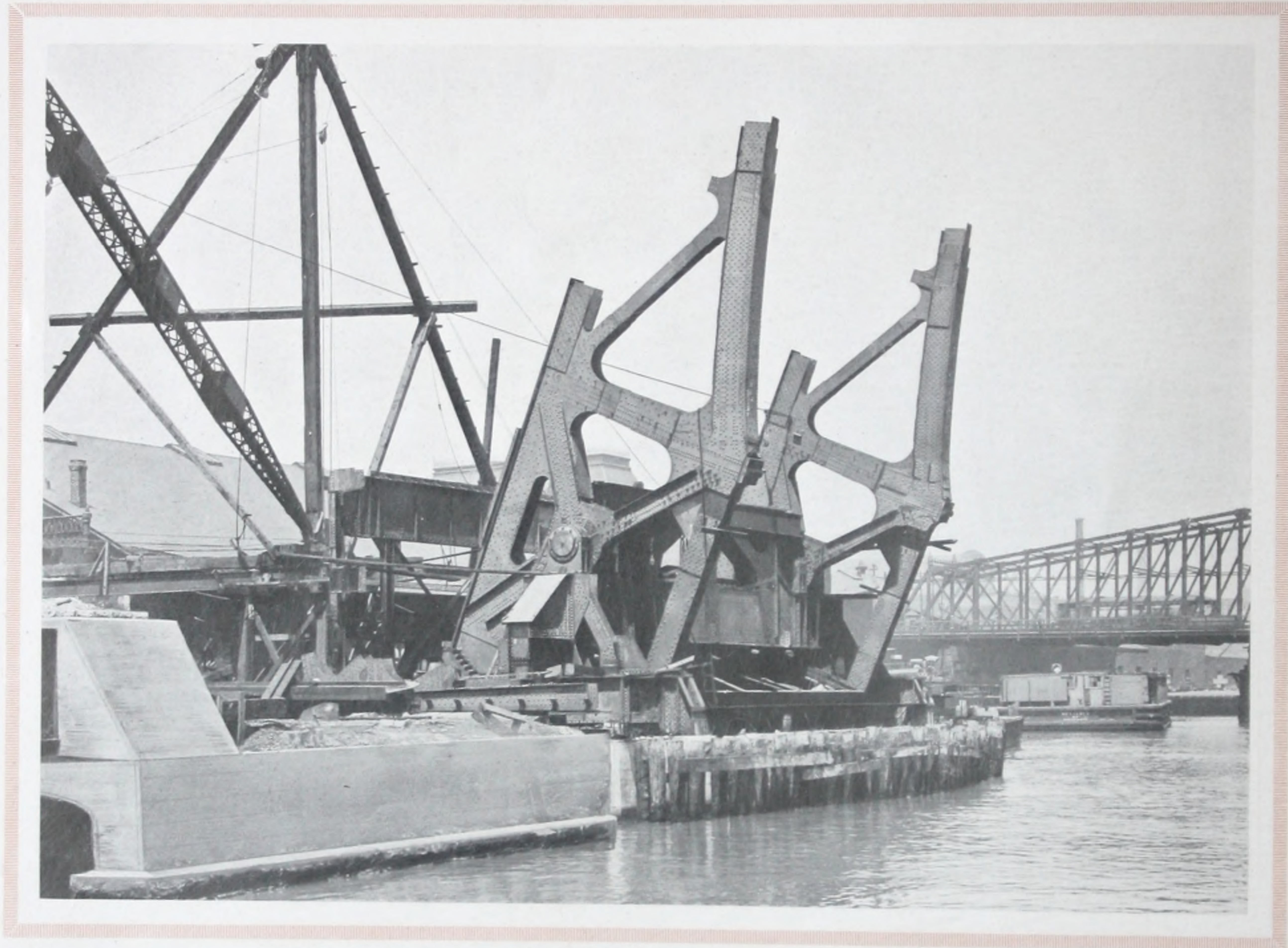
FIGURE 9(c). ERECTION VIEW, JACKSON STREET BRIDGE, CHICAGO
