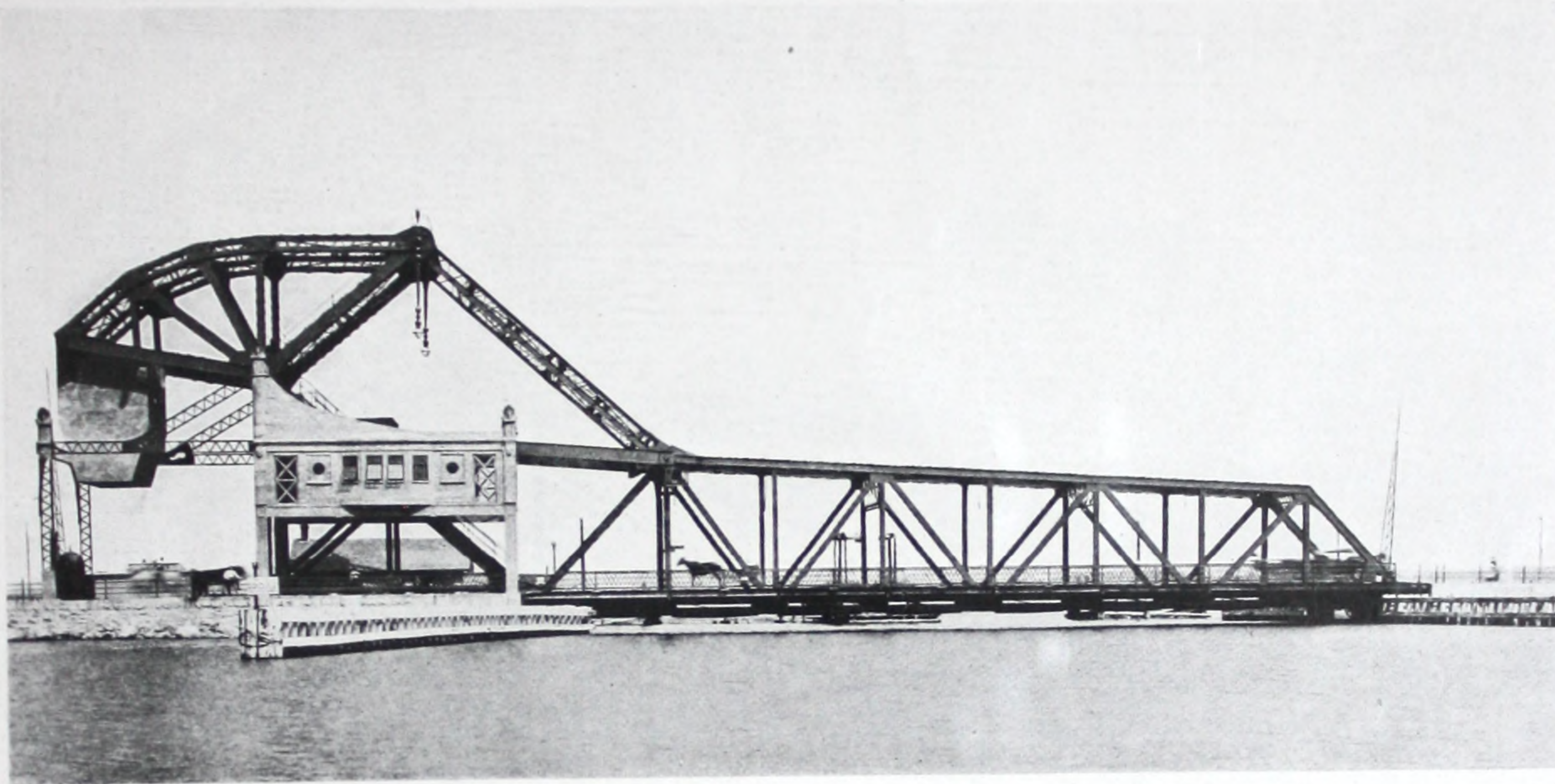
FIGURE 20. SINGLE LEAF HEEL TRUNNION HIGHWAY BRIDGE OVER CATARAQUI RIVER, KINGSTON HARBOR, KINGSTON, ONTARIO Length Bascule span, 170 feet; counterweight span, 42 feet; width roadway, 24 feet; sidewalk, 4 feet. Completed, 1917
