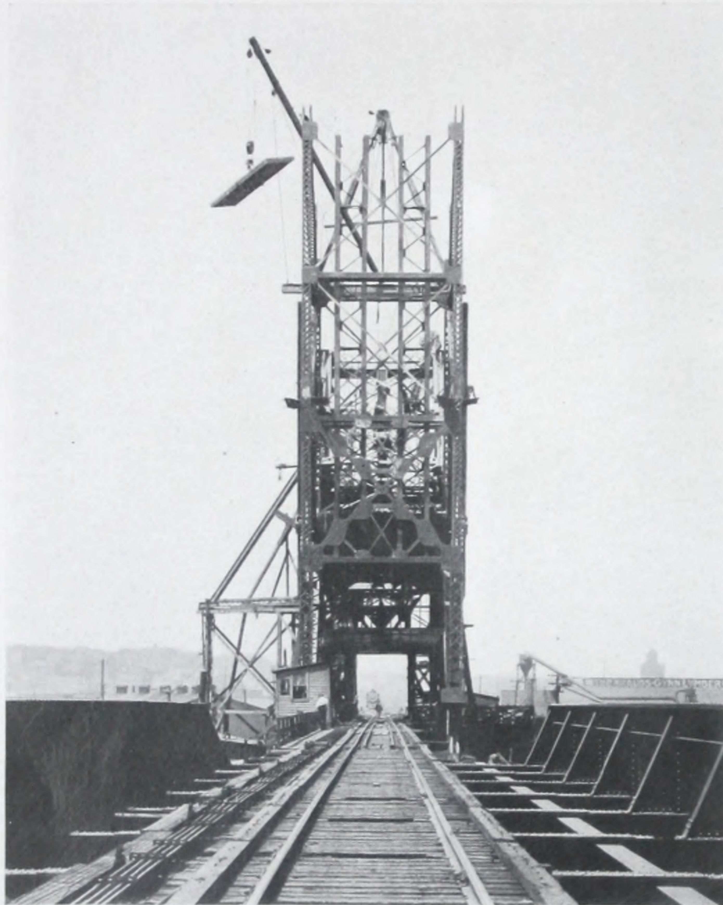
FIGURE 26. ERECTION VIEW ERIE RAILROAD BRIDGE OVER CUYAHOGA RIVER, CLEVELAND, OHIO Length span, 180 feet; double track. Photo taken August, 1911. Bridge completed October, 1911
