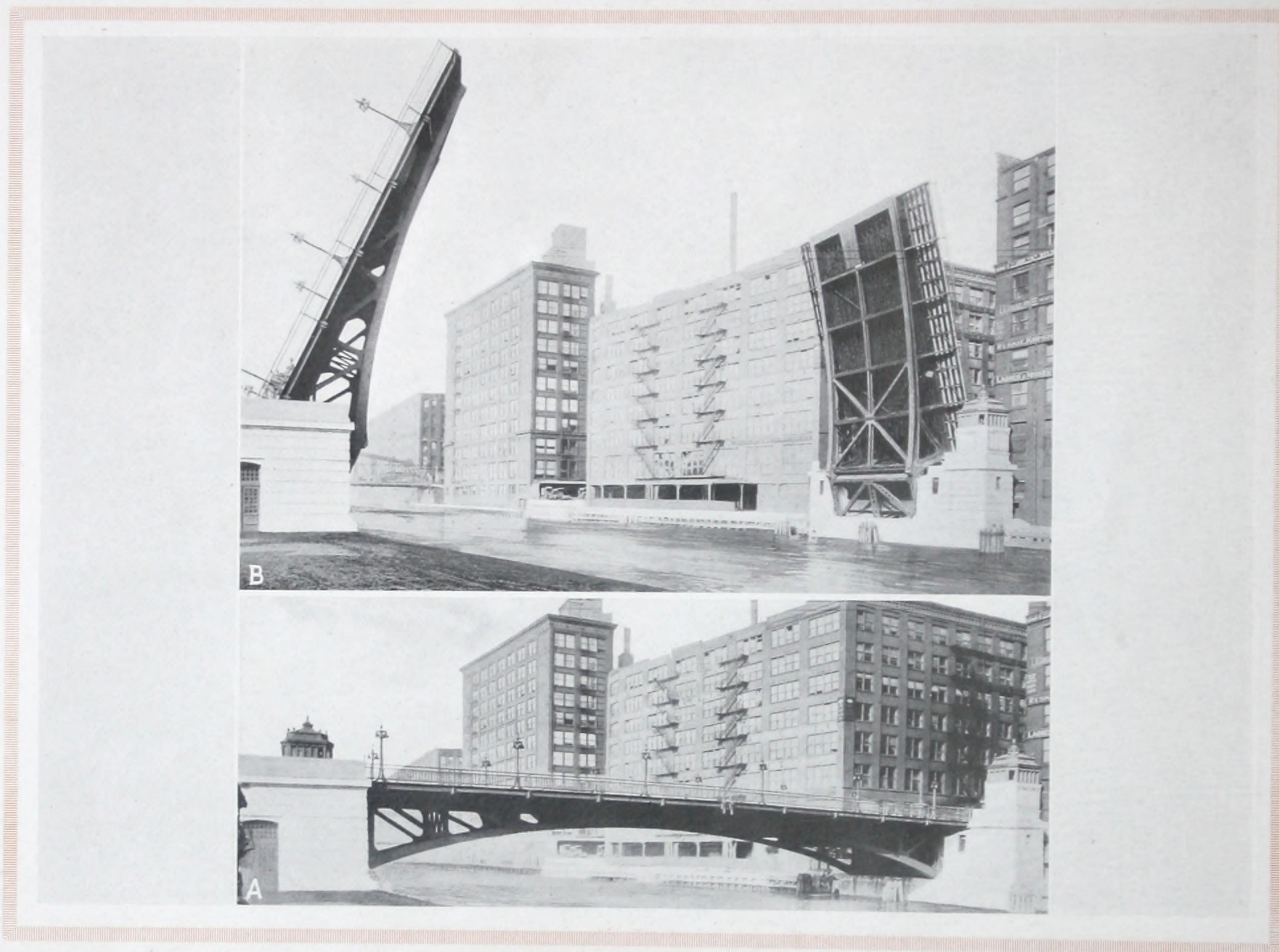
FIGURE 9. (A) AND (B) DOUBLE LEAF UNDERNEATH COUNTERWEIGHT HIGHWAY BRIDGE. JACKSON STREET OVER CHICAGO RIVER, CHICAGO, ILLINOIS Length span, 202 feet; width roadway, 37 feet; sidewalks, 13 feet. Completed, 1916.
