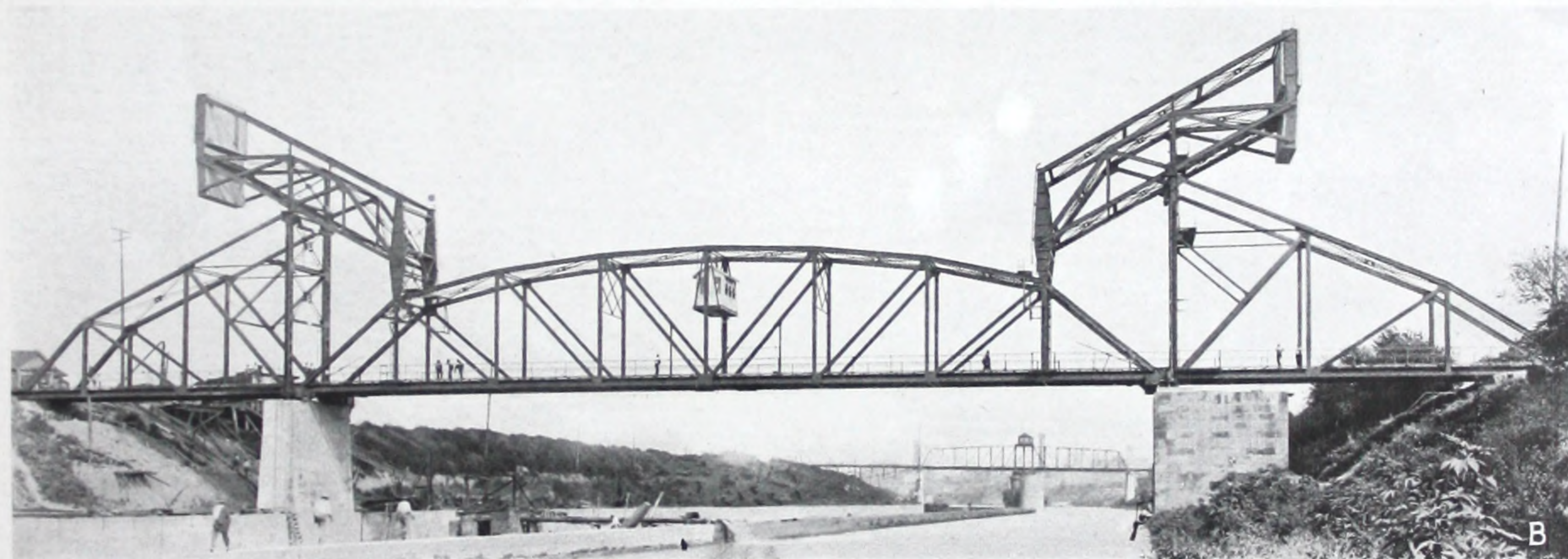
FIGURE 29. DIRECT LIFT HIGHWAY BRIDGE, U. S. GOVERNMENT, OVER LOUISVILLE & PORTLAND CANAL AT 18TH STREET, LOUISVILLE, KENTUCKY
