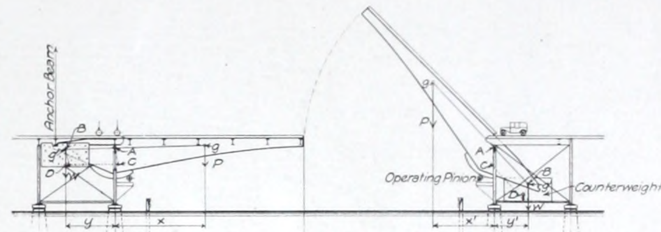
FIGURE 8. DIAGRAM UNDERNEATH COUNTERWEIGHT TYPE.
