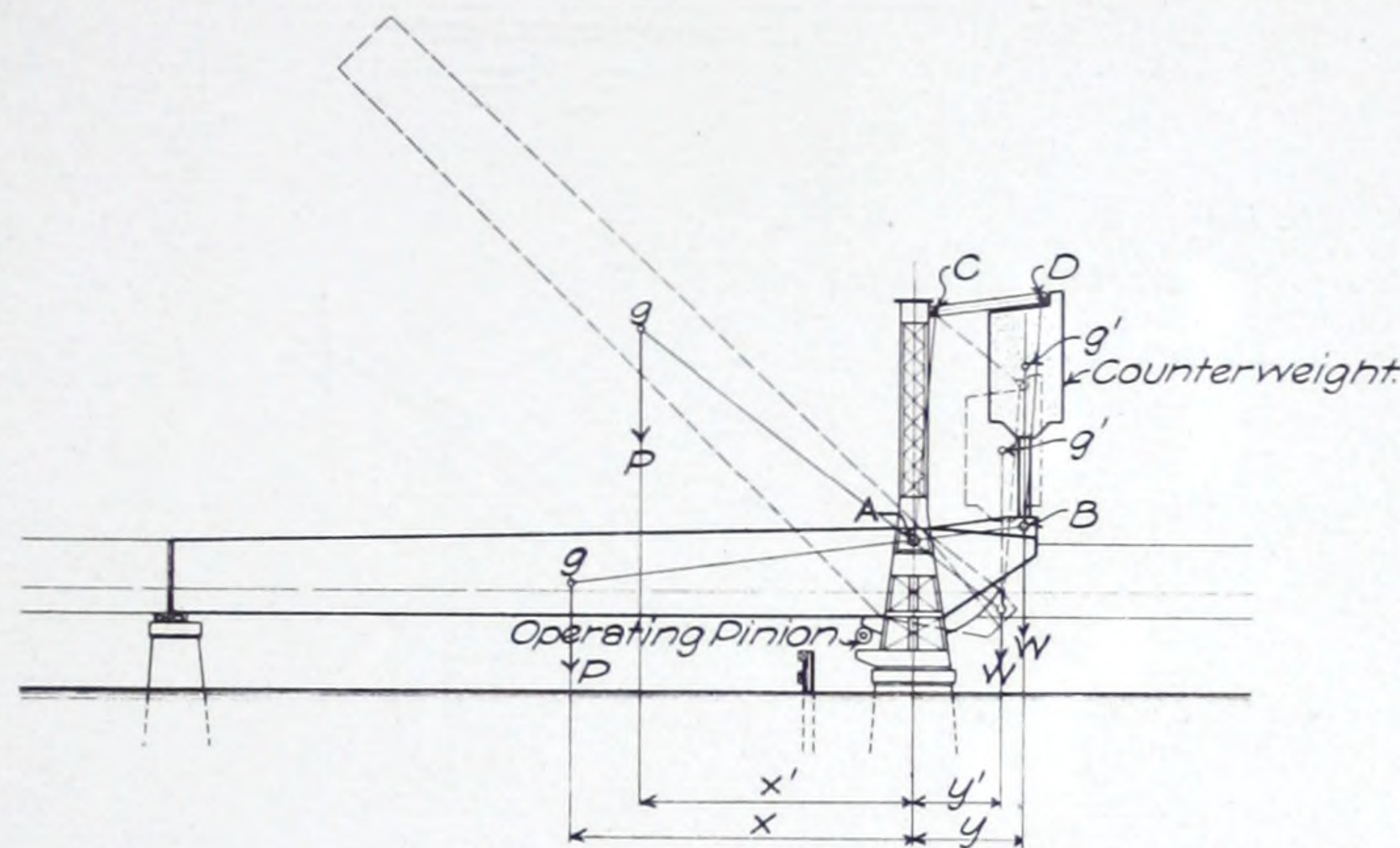
FIGURE 3. DIAGRAM VERTICAL OVERHEAD COUNTERWEIGHT TYPE
