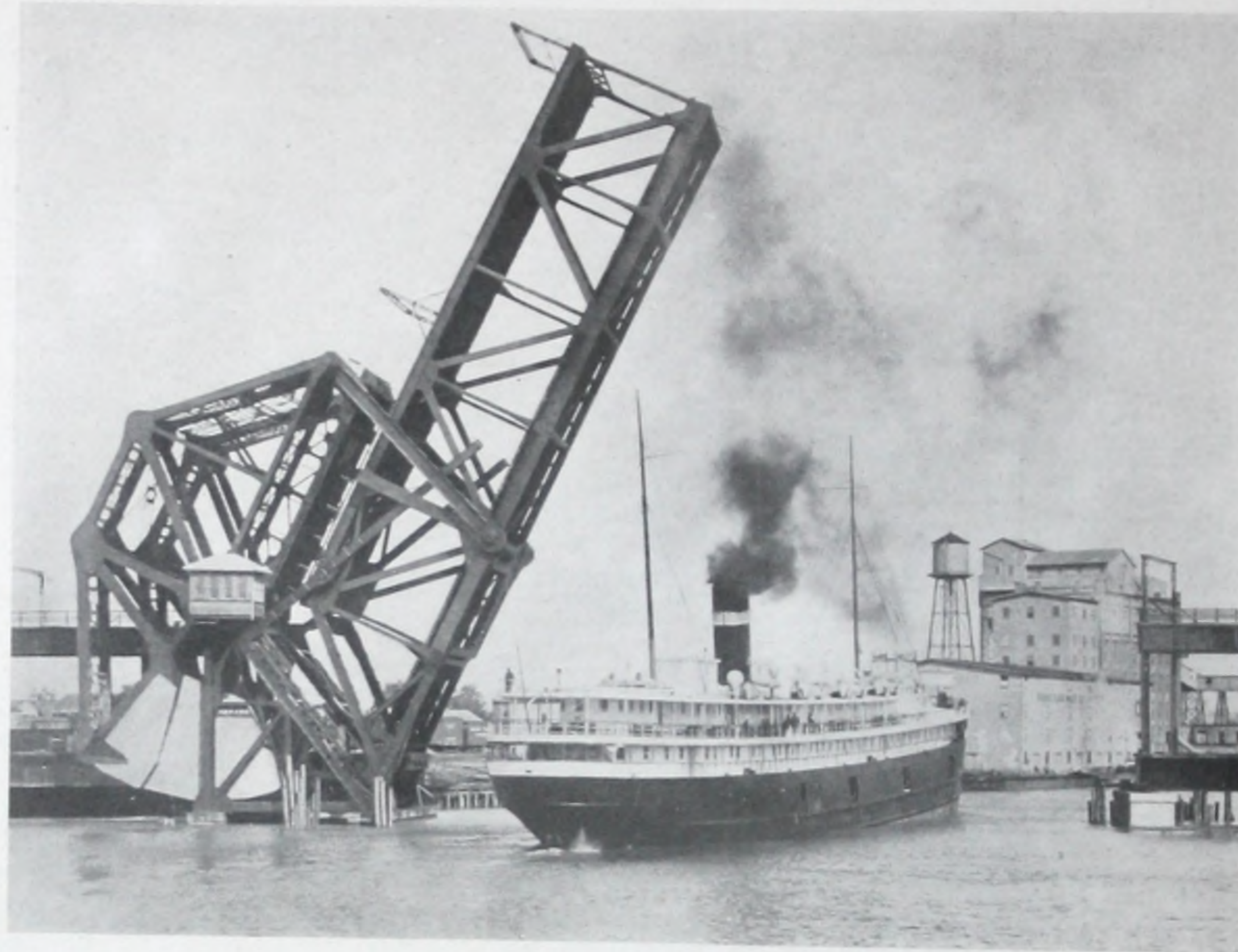
FIGURE 23. DOUBLE DECK SINGLE LEAF HEEL TRUNNION BRIDGE CANADIAN PACIFIC RAILWAY OVER KAMINISTIGUIA RIVER, FORT WILLIAM, ONTARIO Length Bascule span, 186 feet; counterweight span, 40 feet; double track steam railway, lower deck; upper deck, 29 foot clear roadway, double track electric railway. Completed, 1914
