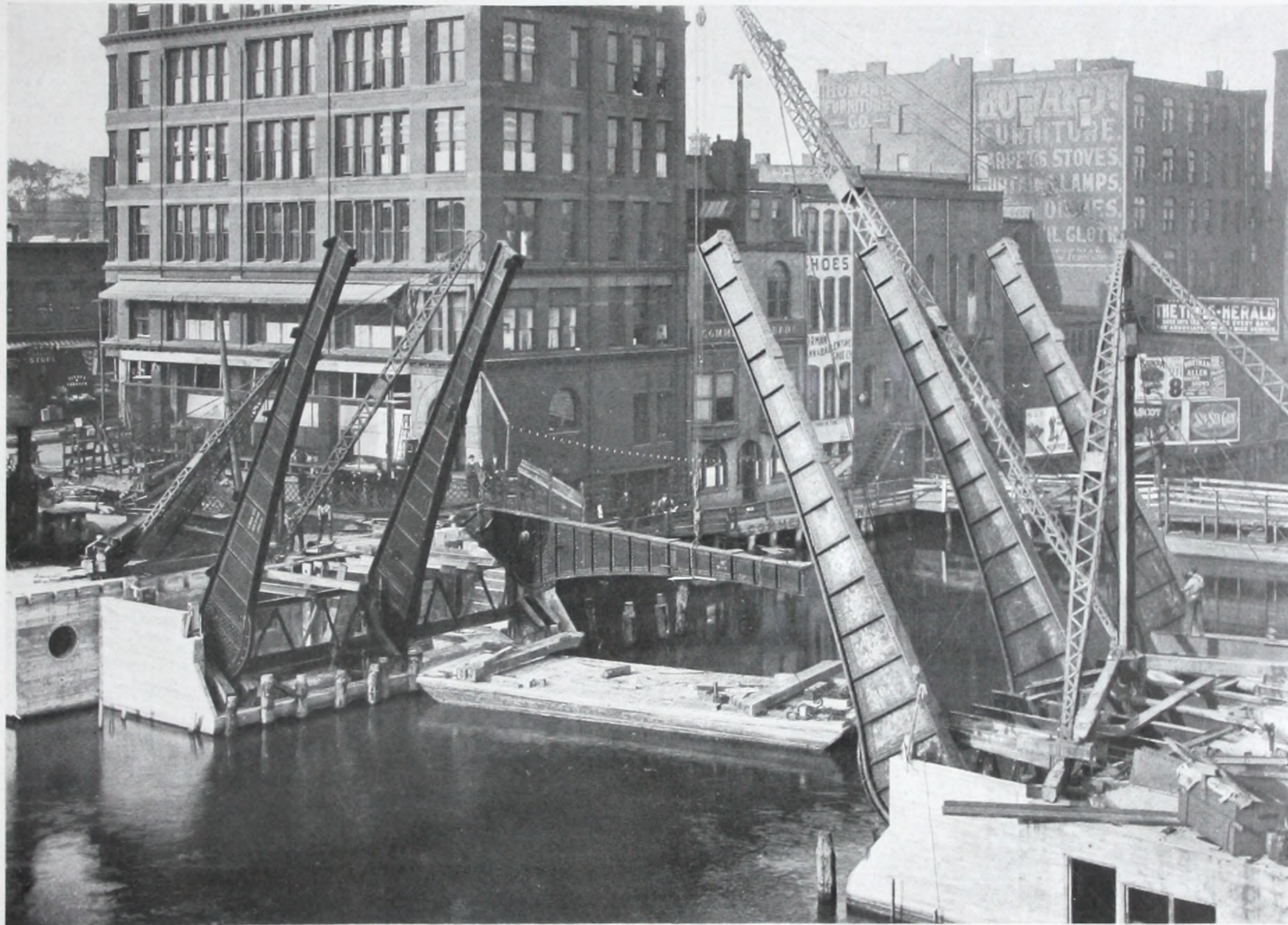
FIGURE 13. ERECTION VIEW MILITARY STREET BRIDGE OVER BLACK RIVER, PORT HURON, MICHIGAN (PHOTOGRAPHED 1913)
