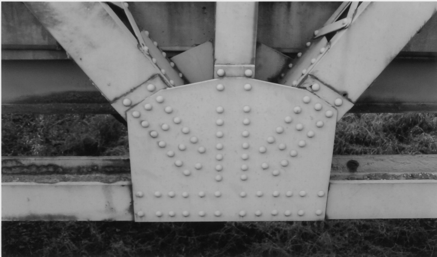
Marion County Bridge 0501F, Marion Co., IN #10
