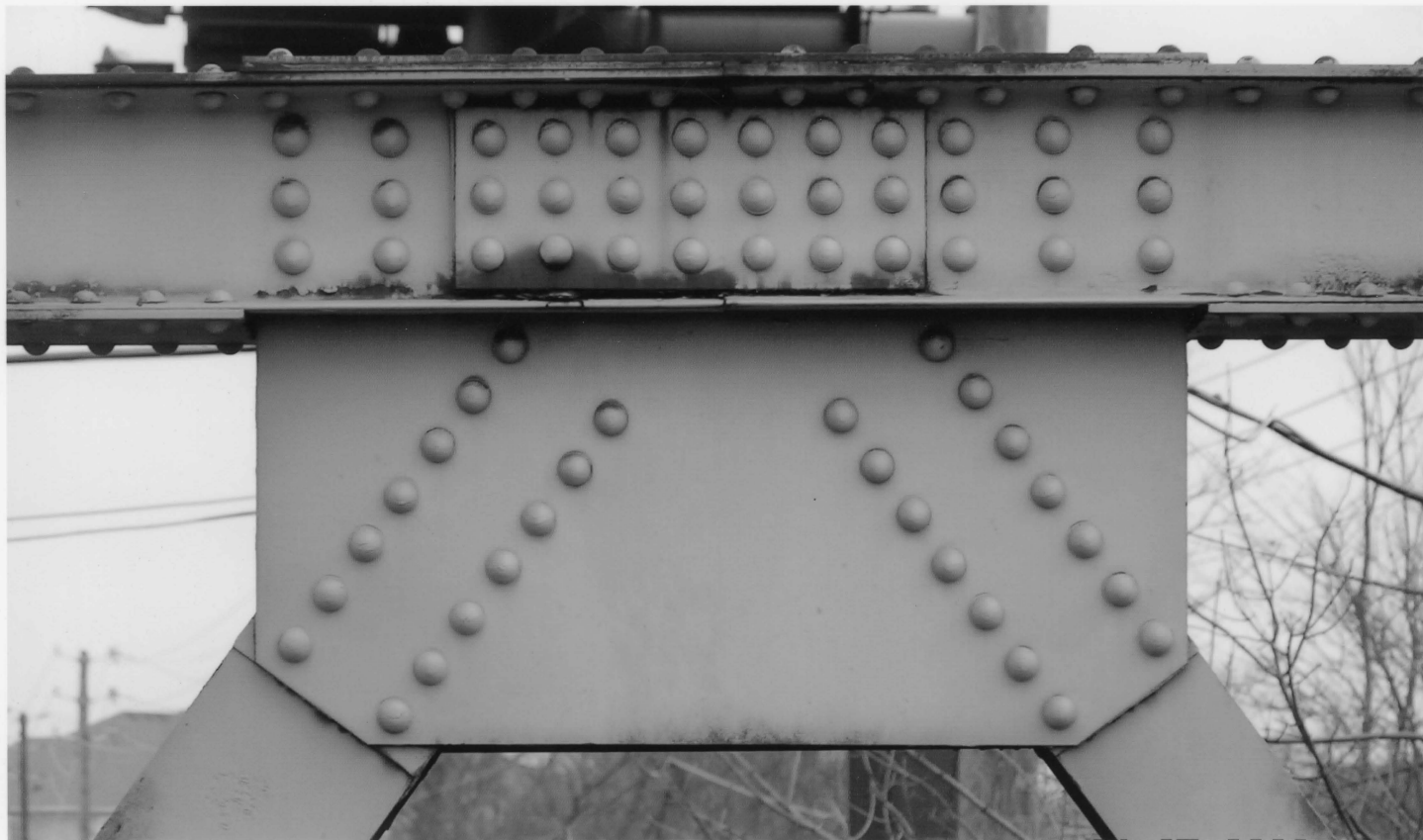
Marion County Bridge 0501F, Marion Co., IN #8
