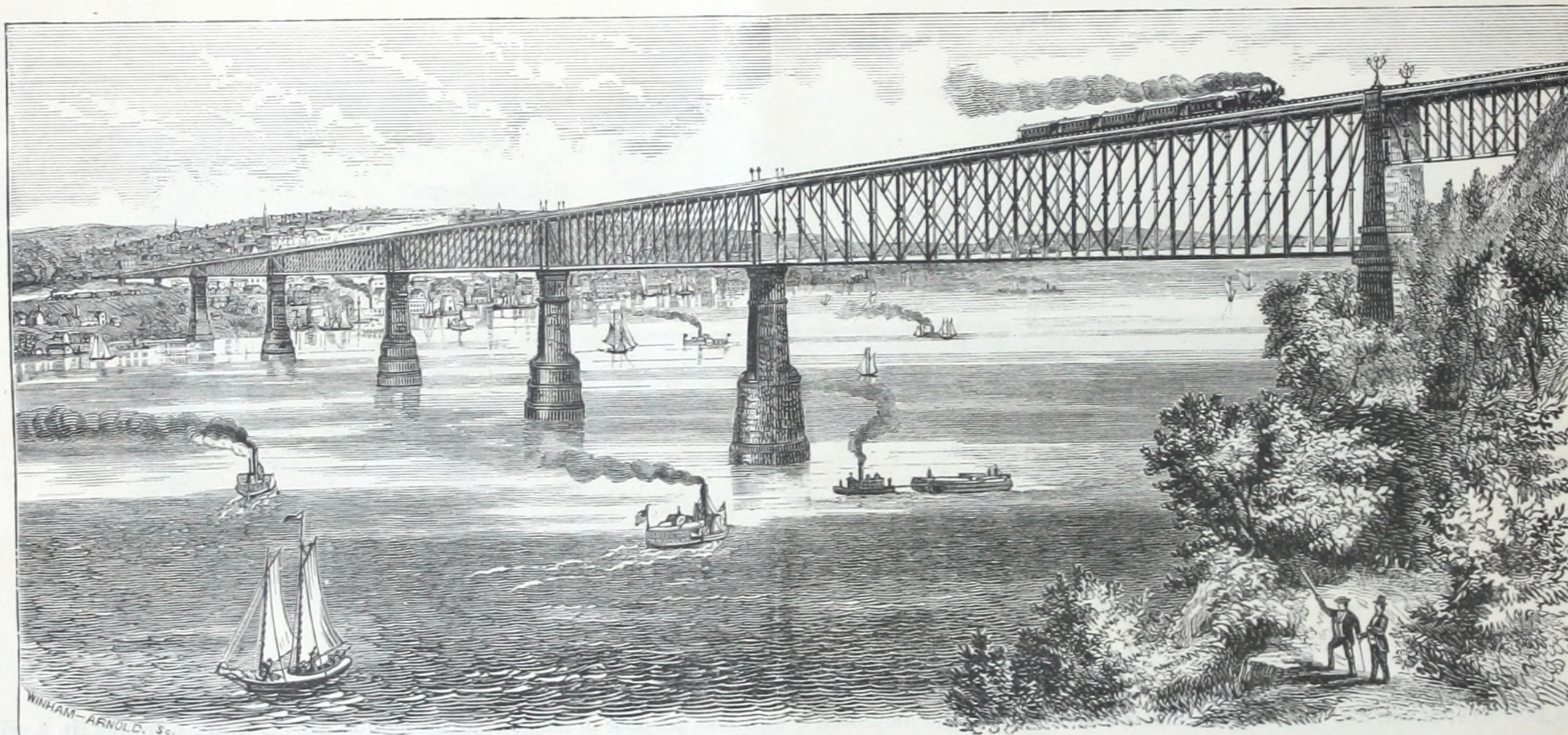
BRIDGE DESIGNED TO CROSS THE HUDSON RIVER, AT POUGHKEEPSIE.
