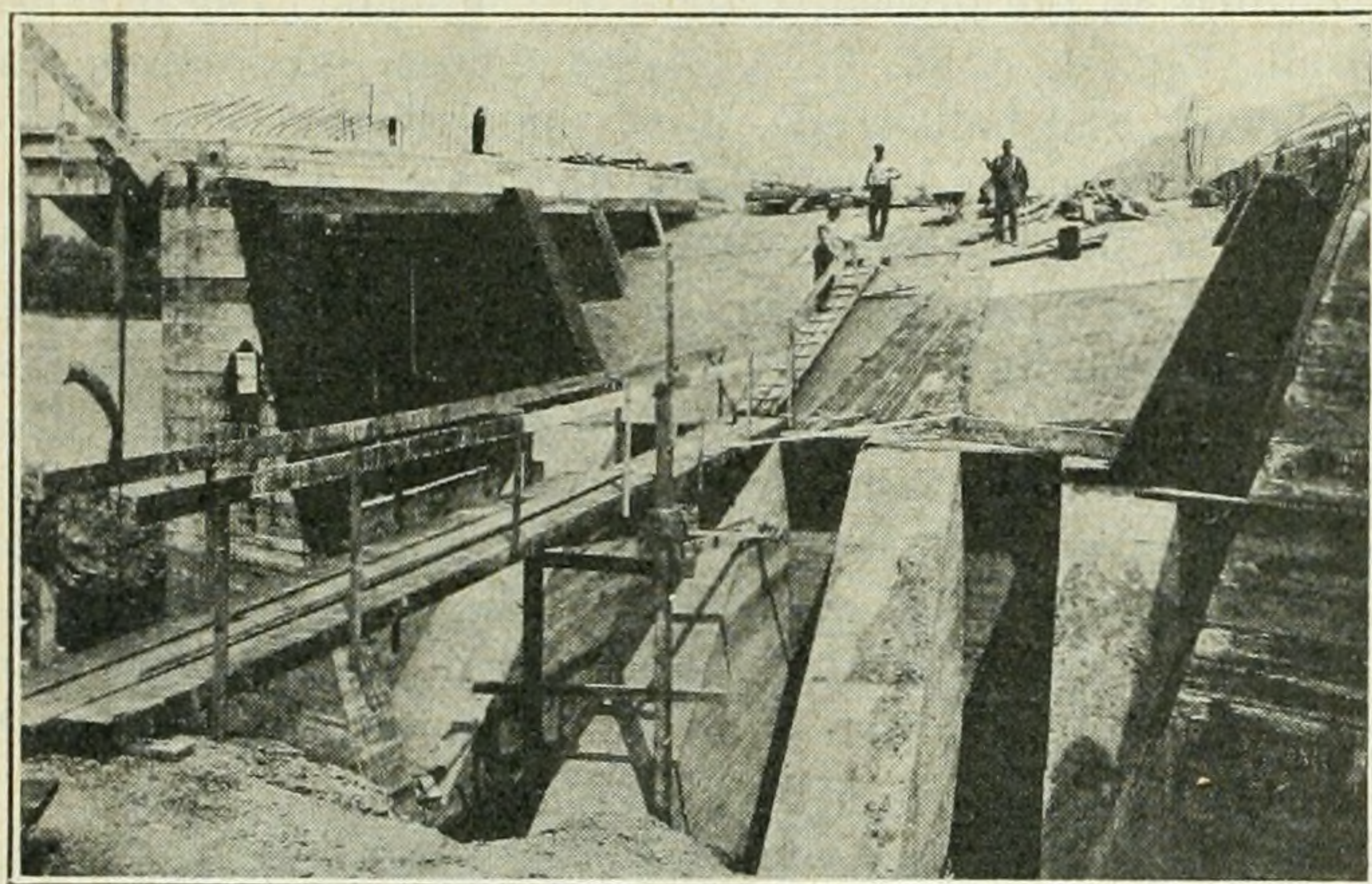
FIG. 5. SOUTH ABUTMENT BUTTRESSES AND WATERPROOFING
