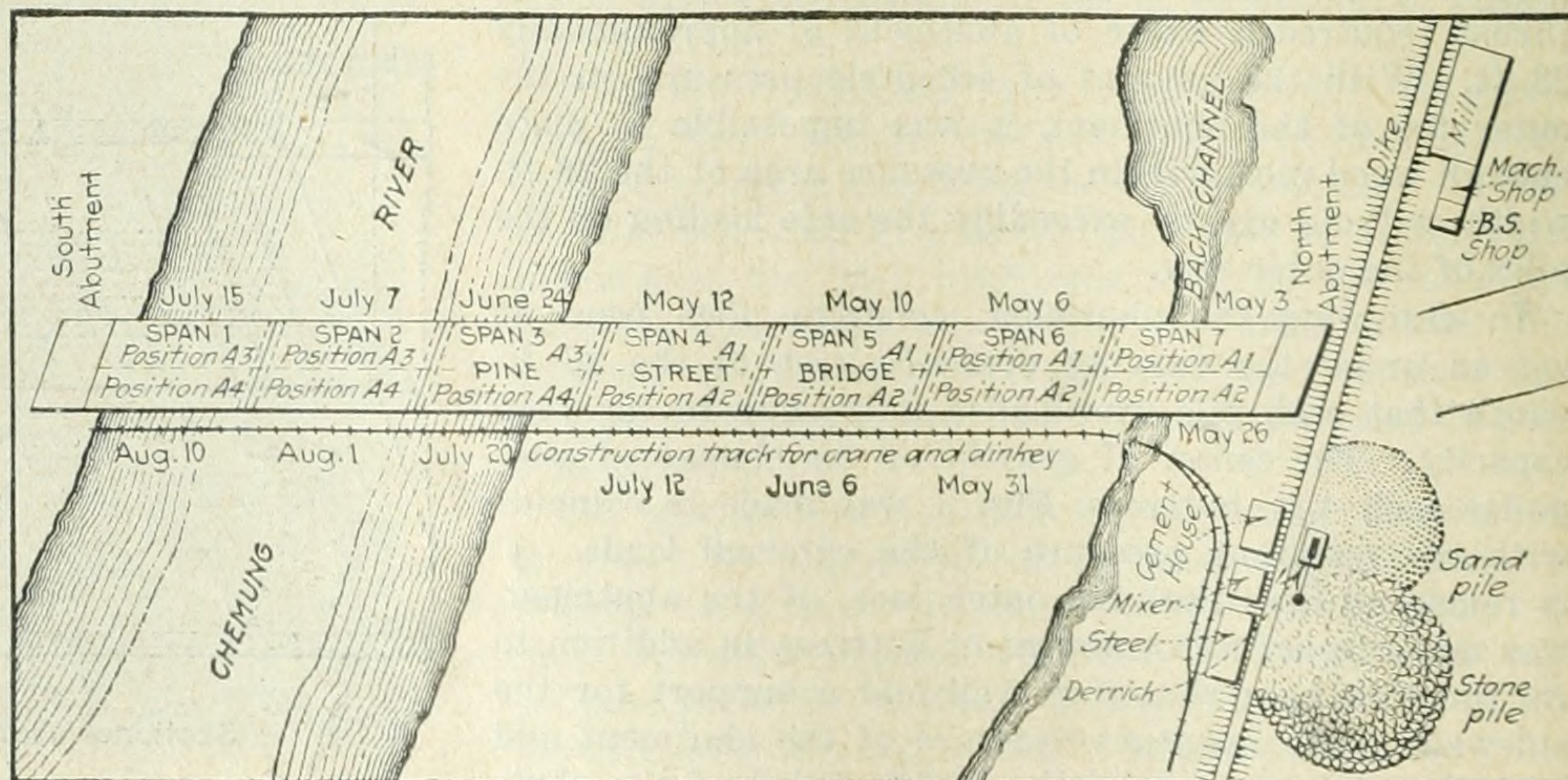
FIG. 6. PLANT LAYOUT AND PROGRESS SCHEDULE
