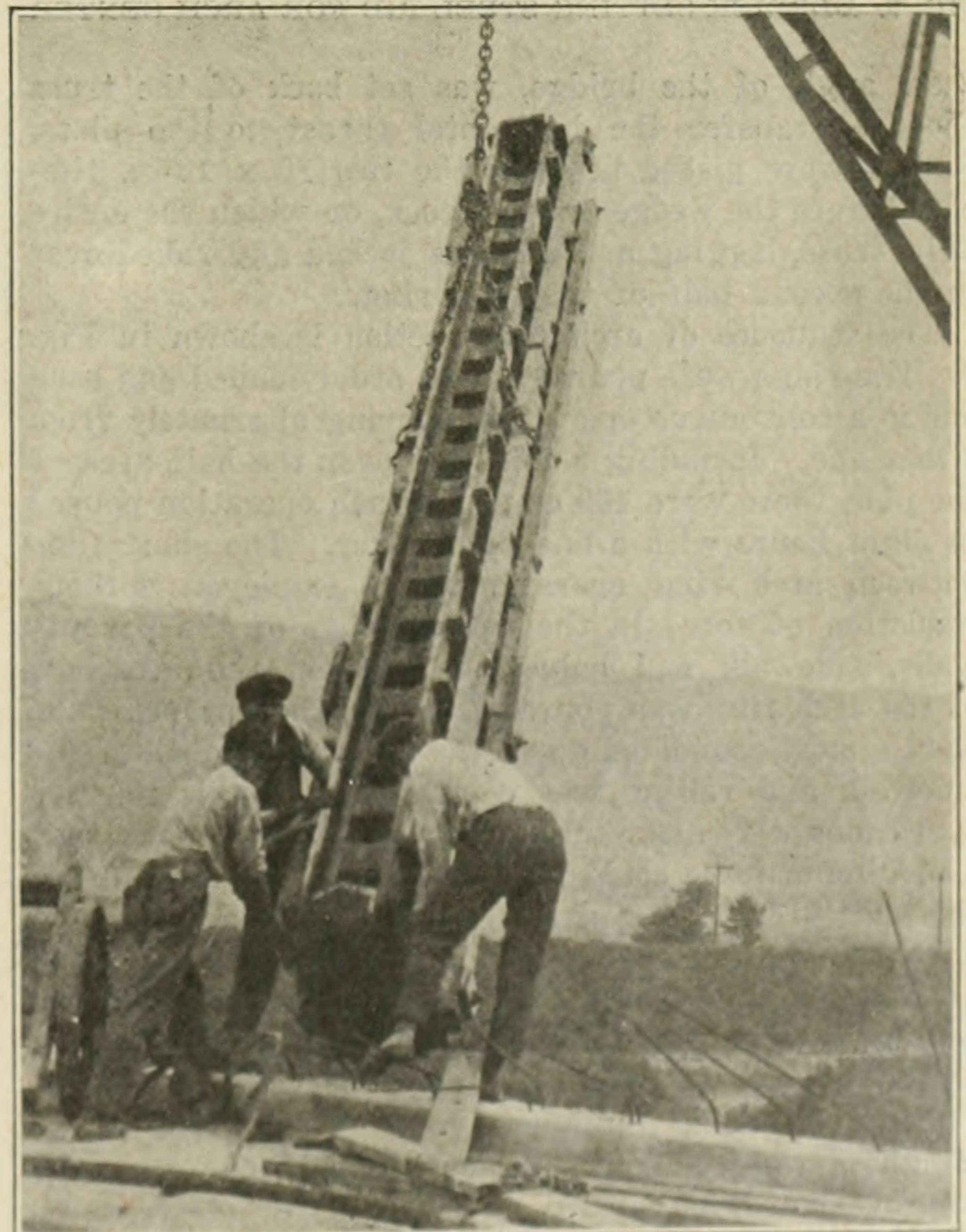
FIG. 7. BALUSTRADE FORM UNITS BEING PLACED
