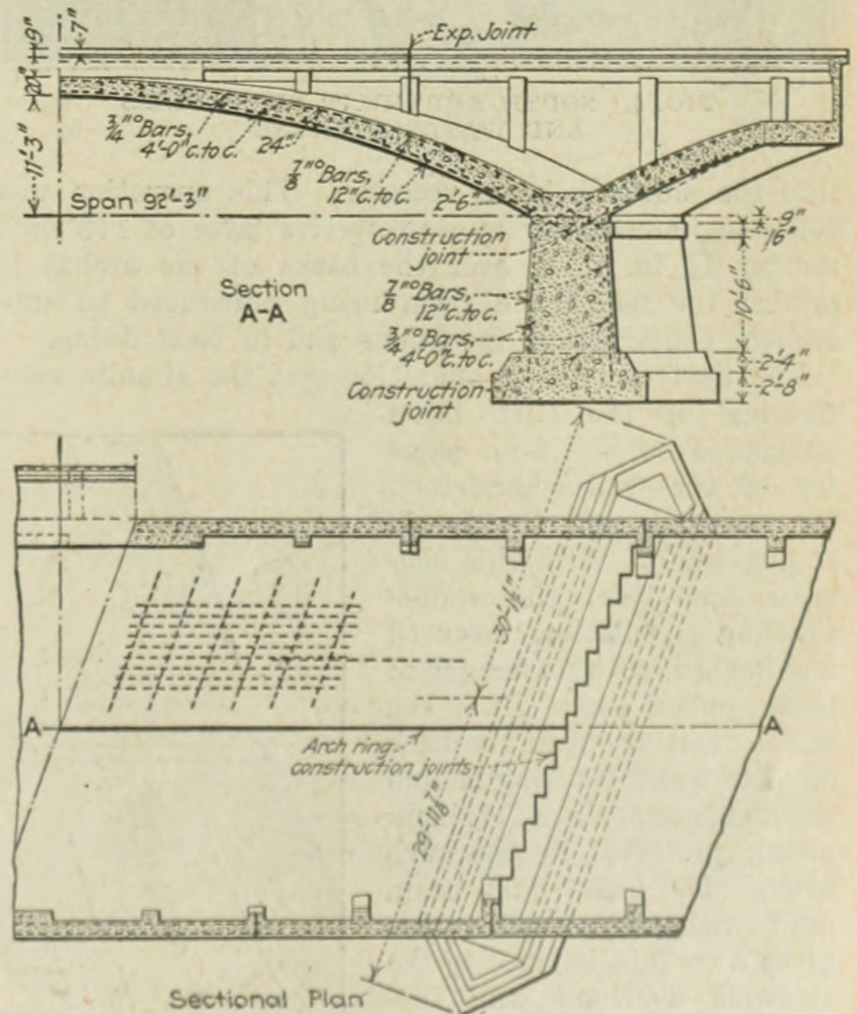
FIG. 3. ARCH SECTION AND PLAN EMPHASIZING CONSTRUCTION JOINTS
