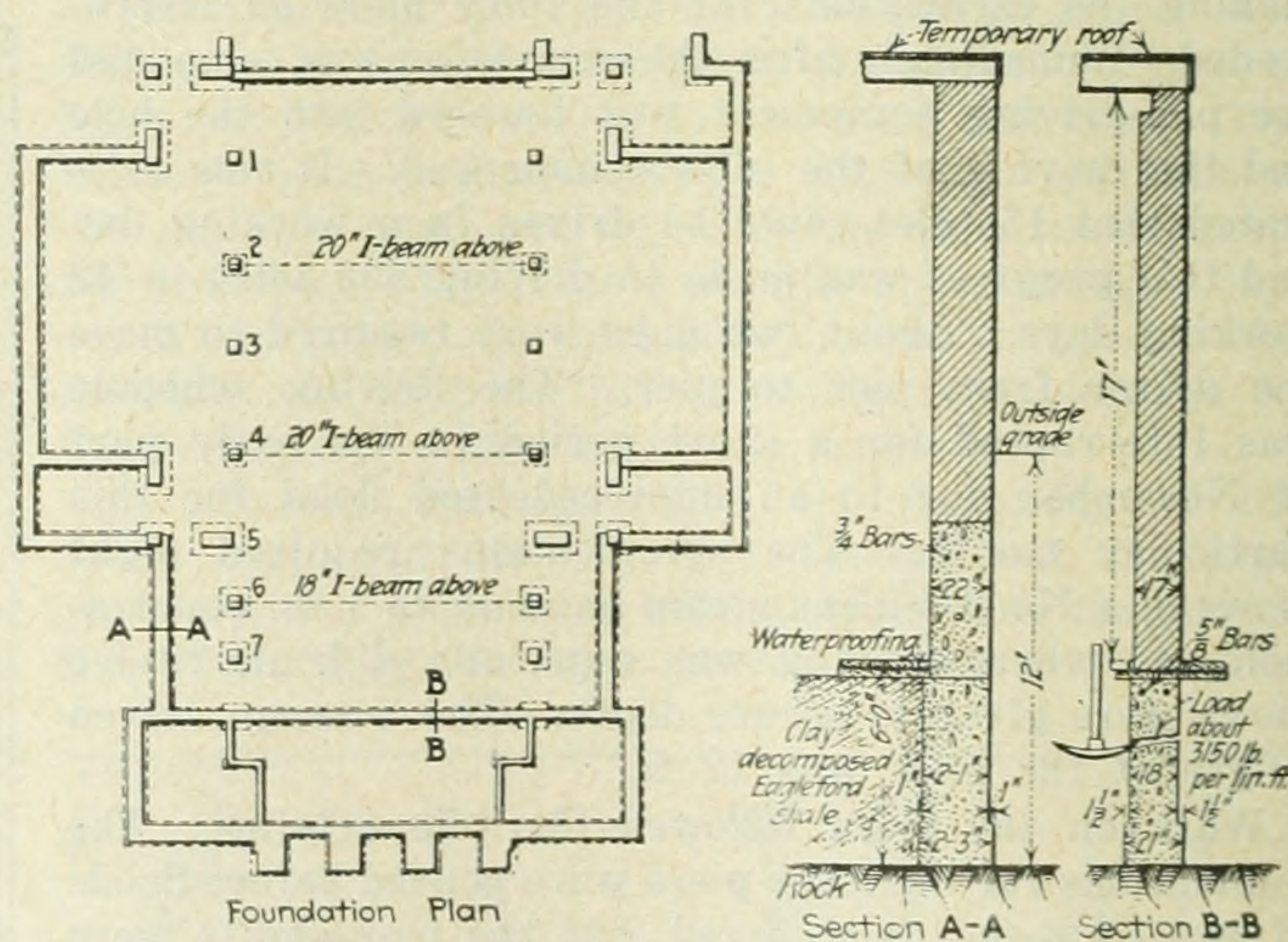
FIG. 1. PLAN OF DAMAGED CHURCH
