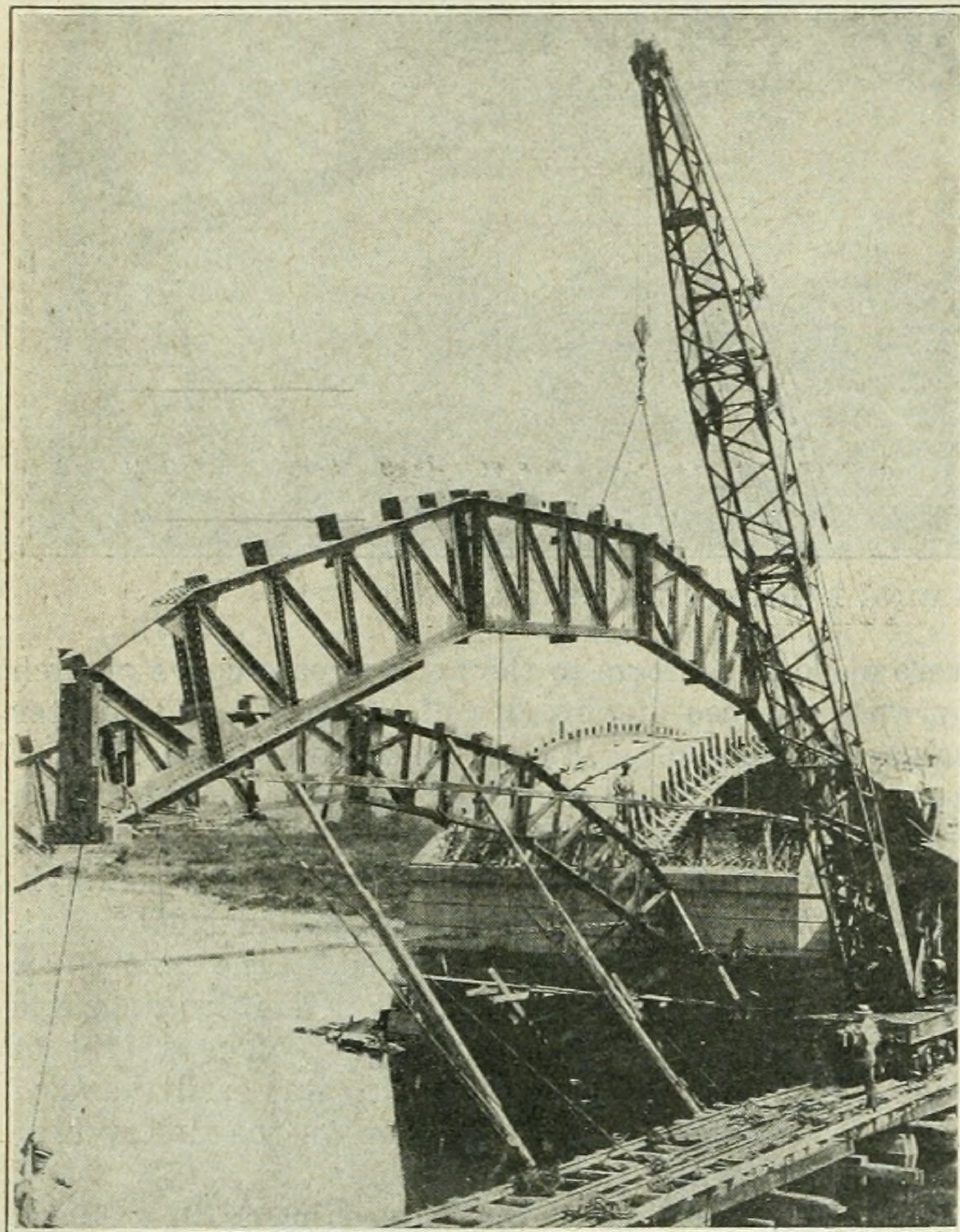
FIG. 9. DERRICK SETTING STEEL RIB FOR ARCH CENTER
