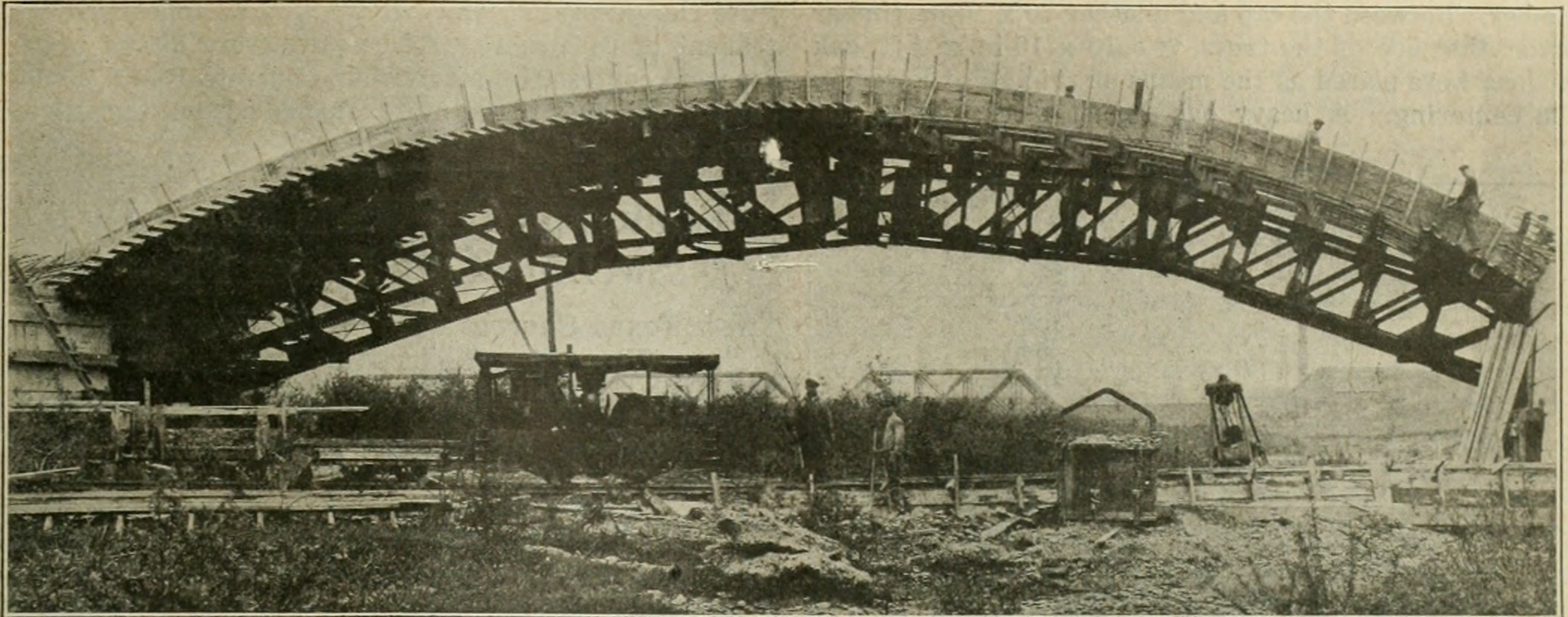
FIG. 8. CENTERS AND ARCH RING FORMS IN PLACE
