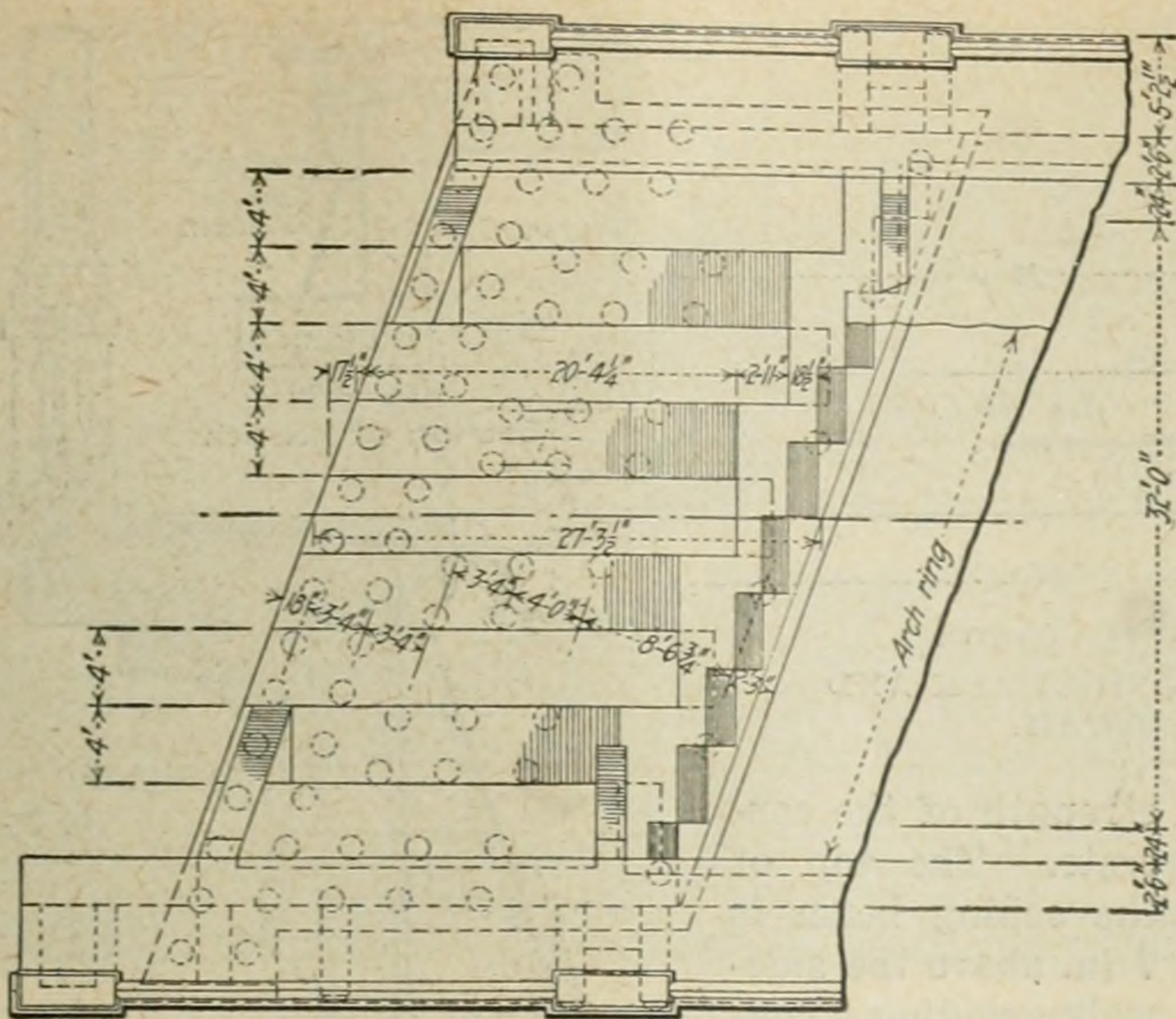
FIG. 2. PLAN OF ABUTMENT SHOWING PILE GROUPING
