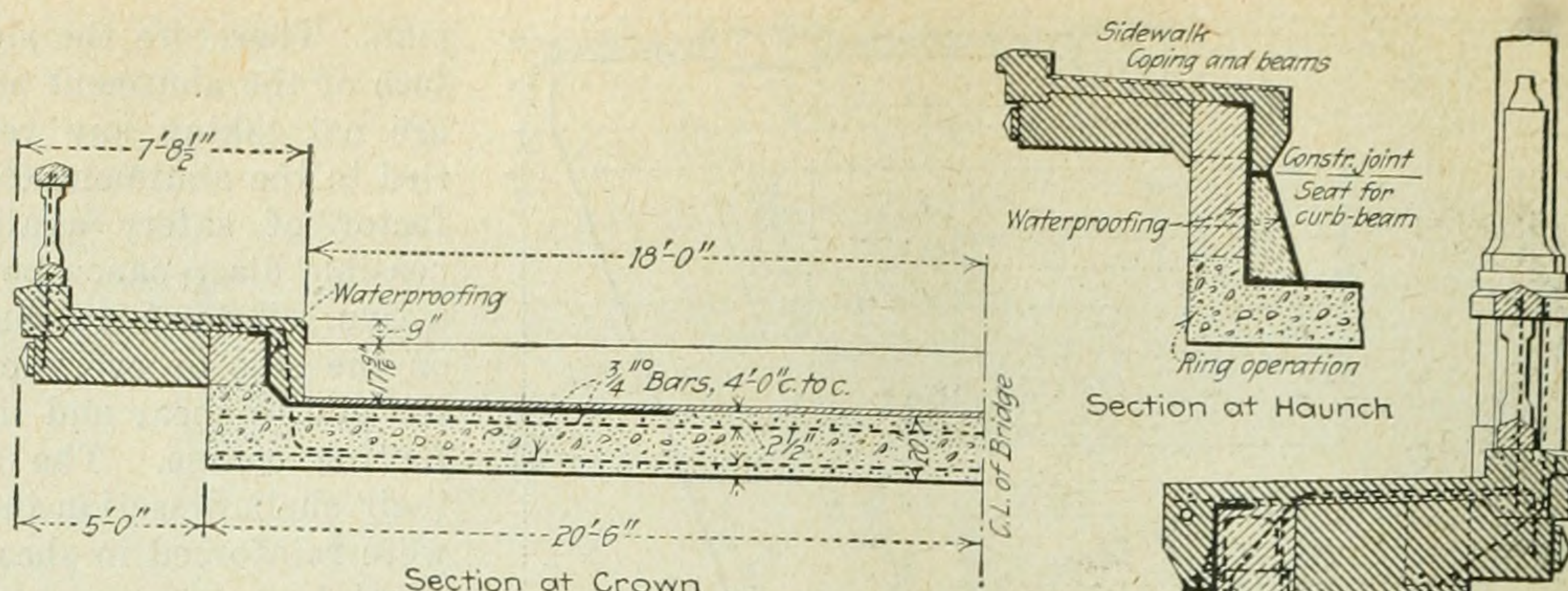
FIG. 4. SPANDREL, SIDEWALK AND PARAPET DETAIL
