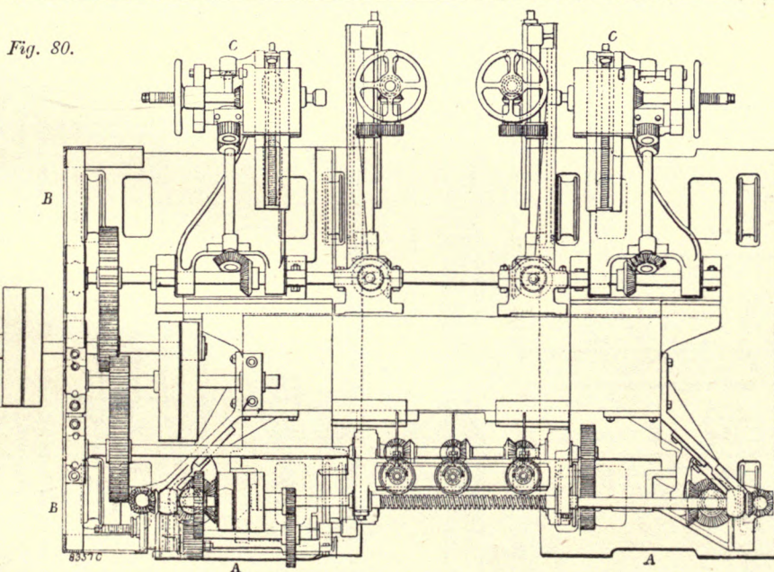
MULTIPLE DRILLING MACHINE; NO. 1 SHED.
