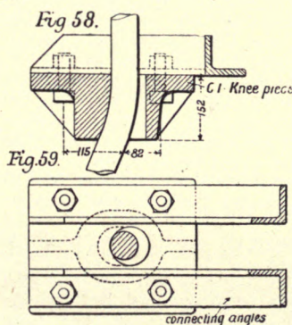
MODE OF FIXING UNDER BEDPLATES ON PIERS.
