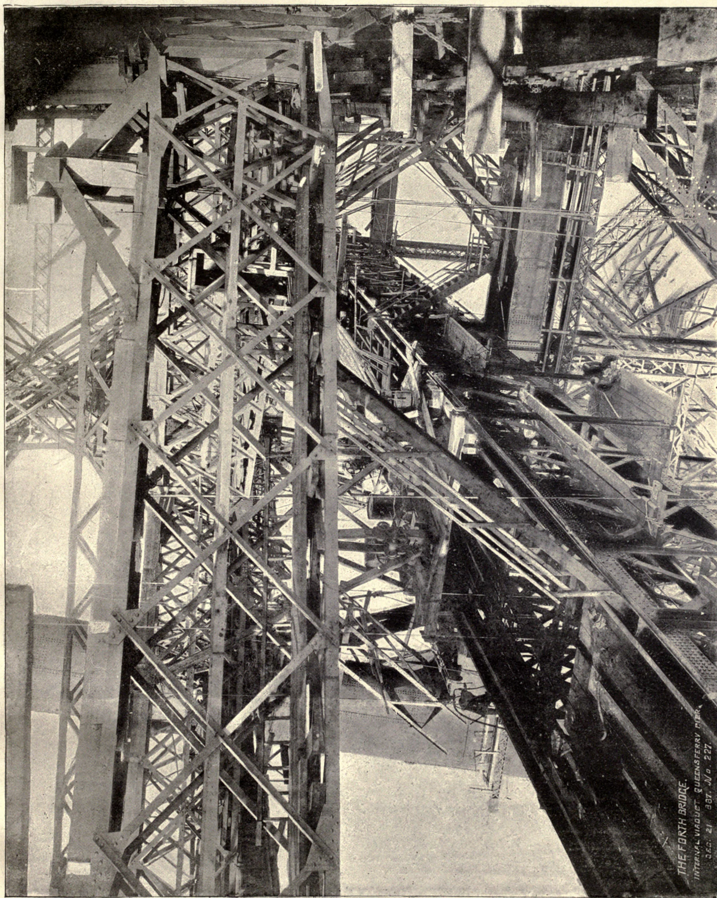
QUEENSFERRY PIER. INTERNAL VIADUCT FROM CENTRE OF BAY TO WITHIN CENTRAL TOWERS.
