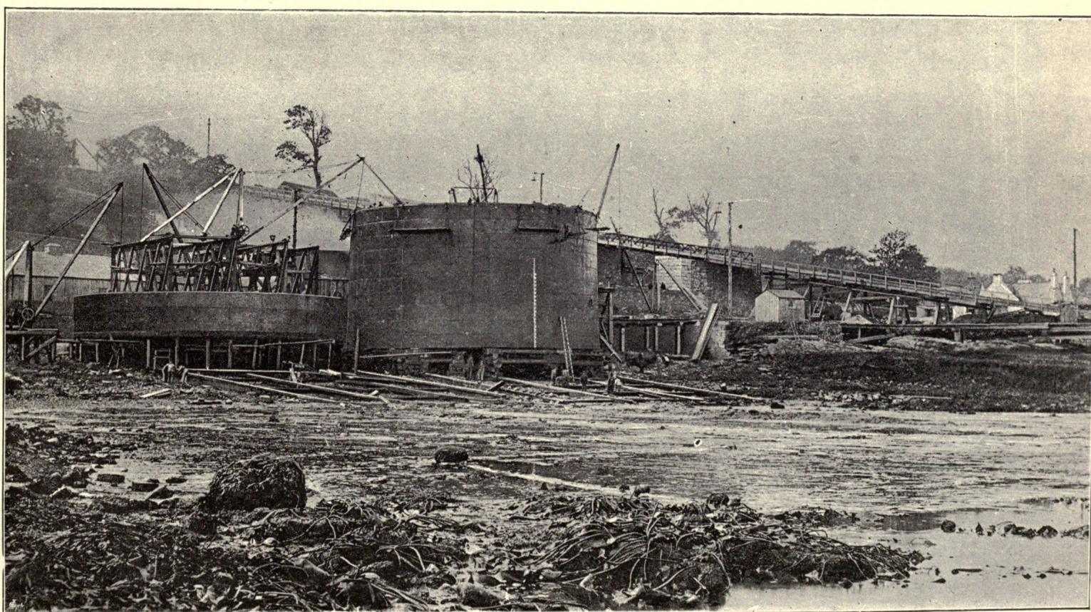
CAISSONS BUILDING ON LAUNCHING WAYS.
