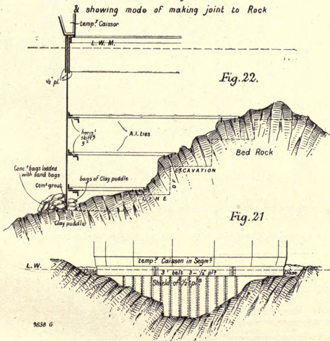
INCH-GARVIE IRON COFFER-DAM. N.W. PIER.
