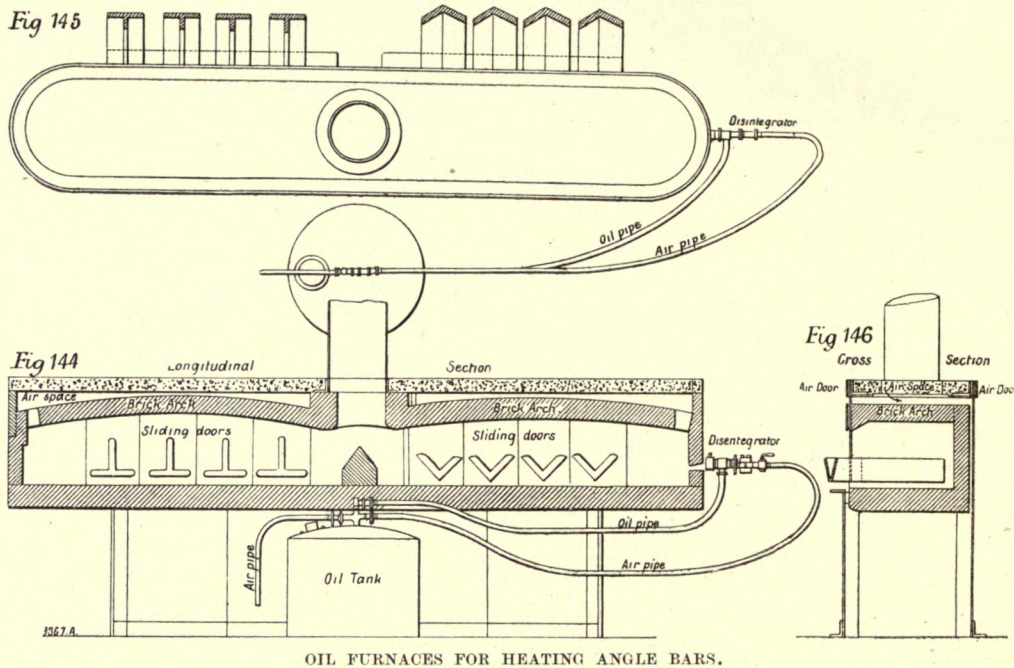
OIL FURNACES FOR HEATING ANGLE BARS.
