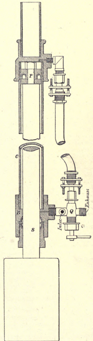
HYDRAULIC SPADE.
