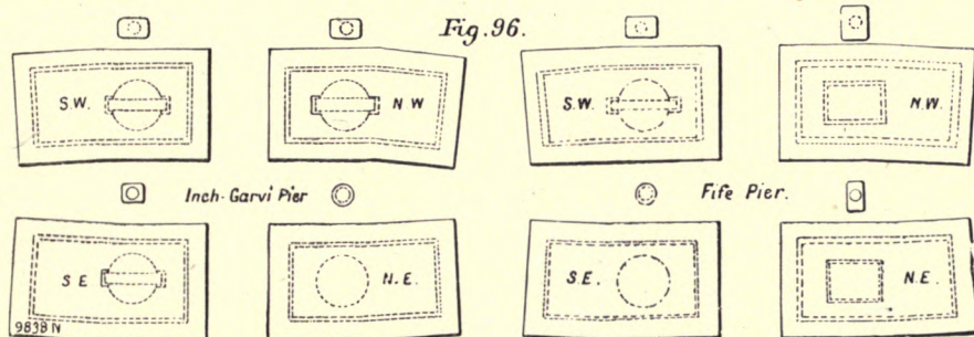
BEDPLATES ON INCHGARVIE AND FIFE PIERS.
