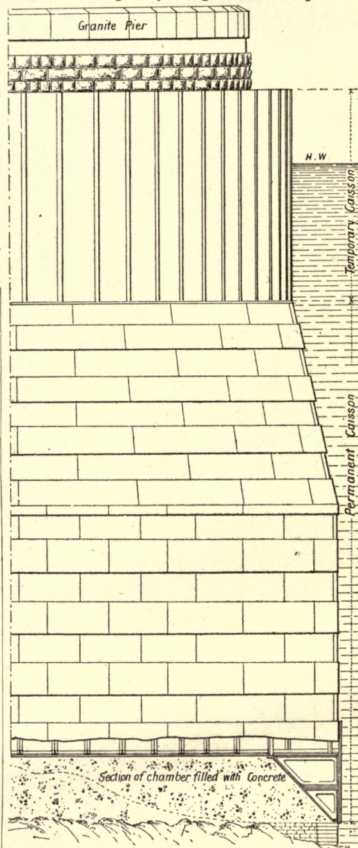
FIG. 53. PIER WITH PERMANENT CAISSON.
