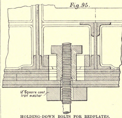
HOLDING-DOWN BOLTS FOR BEDPLATES.
