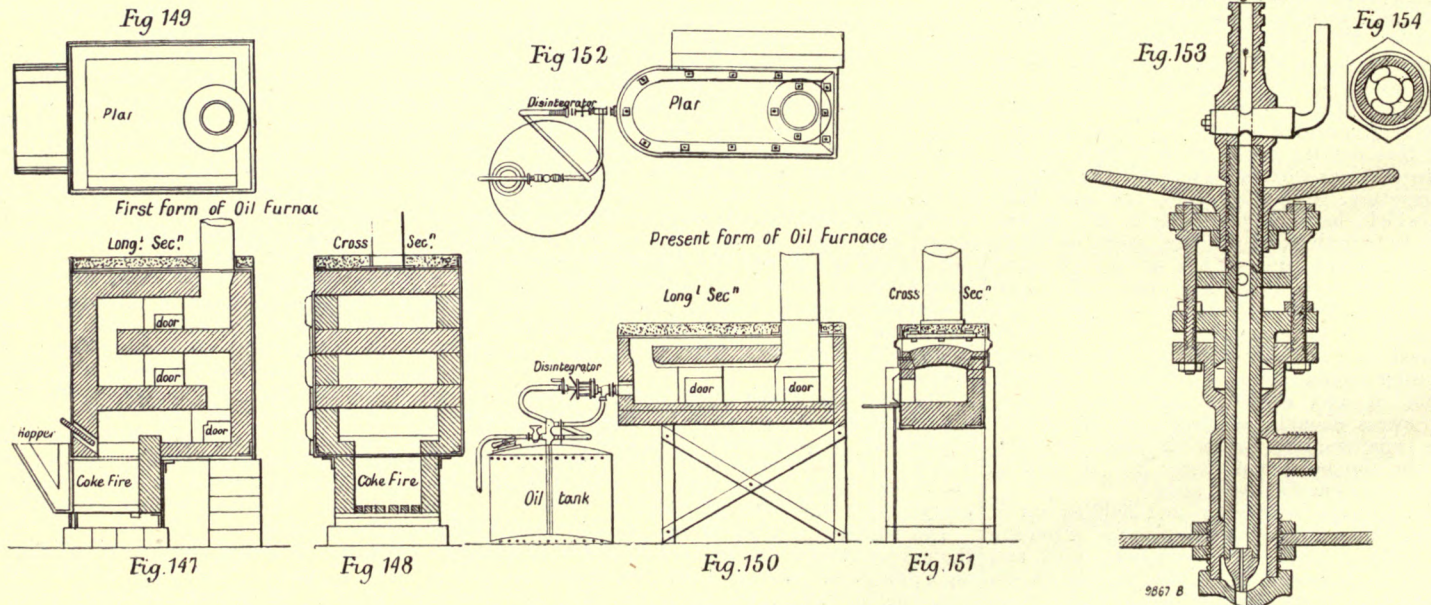
OIL FURNACES FOR HEATING RIVETS.
