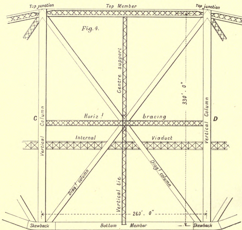
Central Tower
