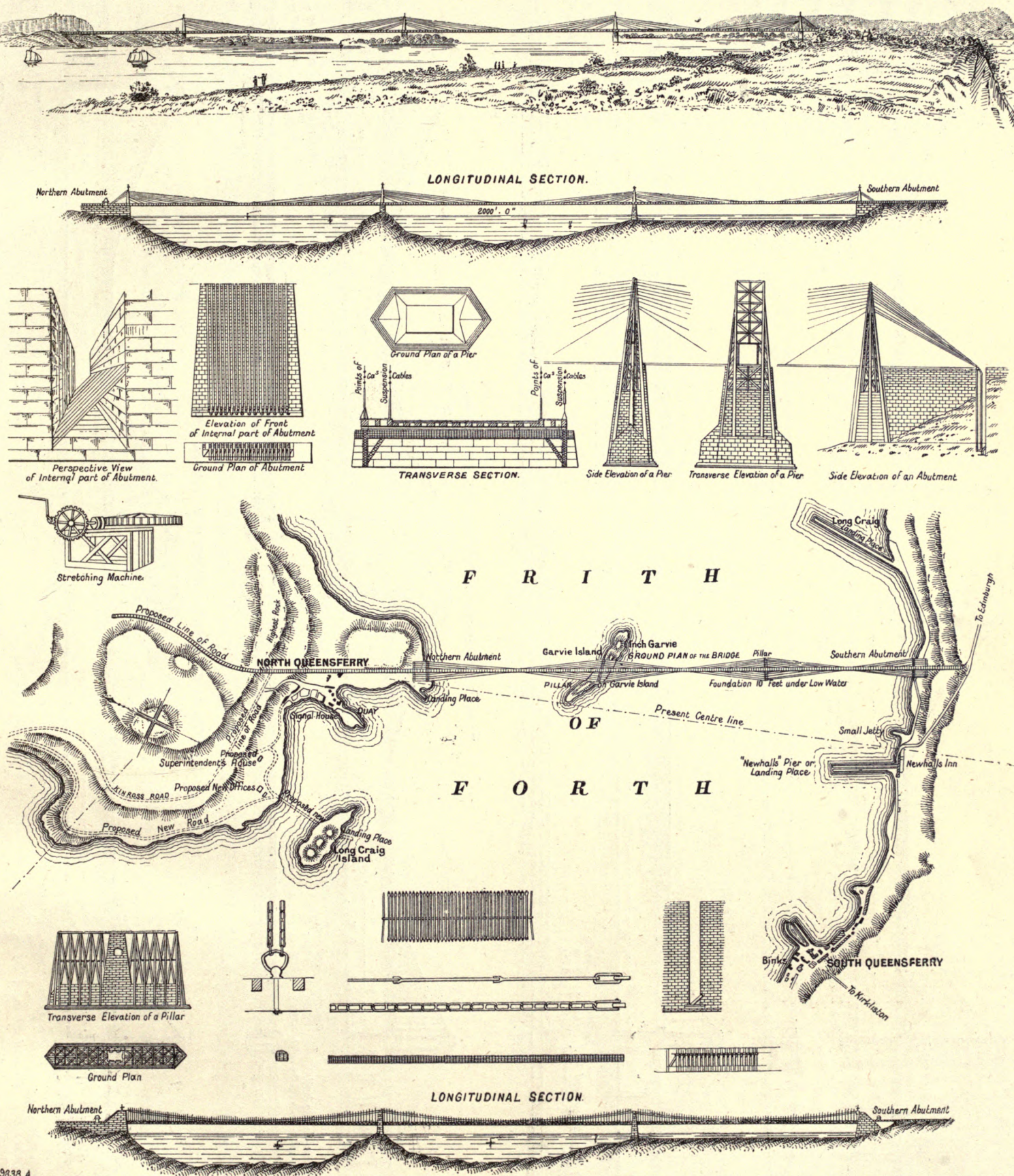
FIG. 1. ANDERSON'S DESIGN FOR BRIDGE OVER THE FORTH, 1818.
