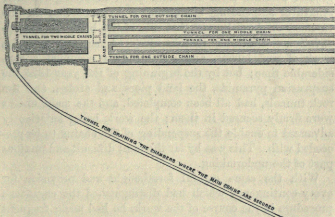
CUT SHOWING FIXING OF THE CHAINS IN THE ROCK.
