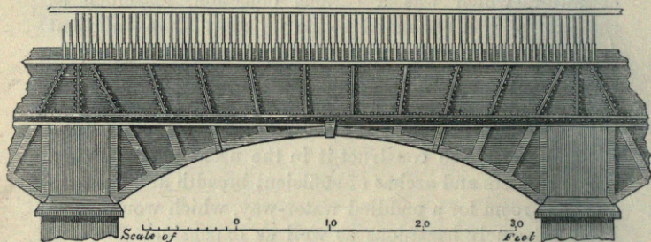
PONT-CYSYLLTAU—SIDE VIEW OF CAST IRON TROUGH.
