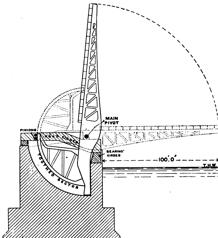
FIG. S. DIAGRAM OF BASCULE TO SHOW QUADRANT OR SECTOR.
