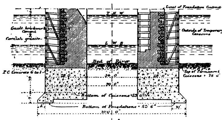
FIG. M. CROSS SECTION OF PIER SHOWING OUTSIDE WALL COMPLETED.
