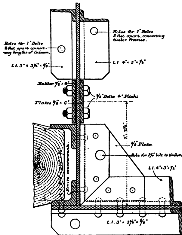
DETAIL OF VERTICAL JOINTS AND PILE GROOVES
