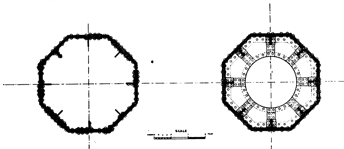
FIG. Y. PLANS OF MAIN PILLARS.
