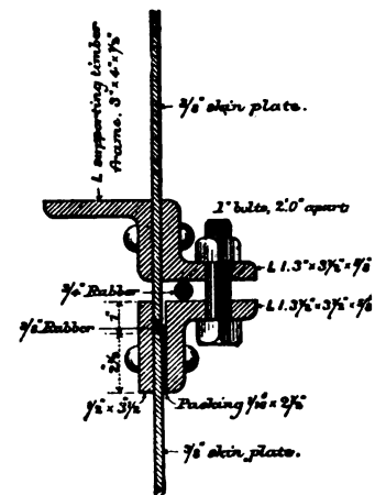
DETAIL OF INDIA-RUBBER JOINT.
