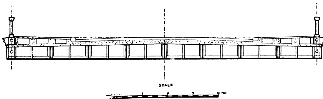
FIG. BB. CROSS SECTION OF PLATFORM OF SUSPENSION SPANS.
