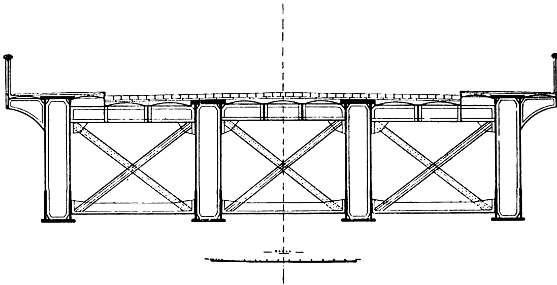
FIG. Q. CROSS SECTION OF LEAF OF OPENING SPAN.
