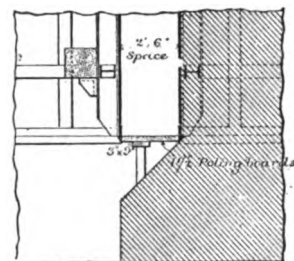
SHOWING UNDERCUTTING BETWEEN TWO ADJOINING CAISSONS.
